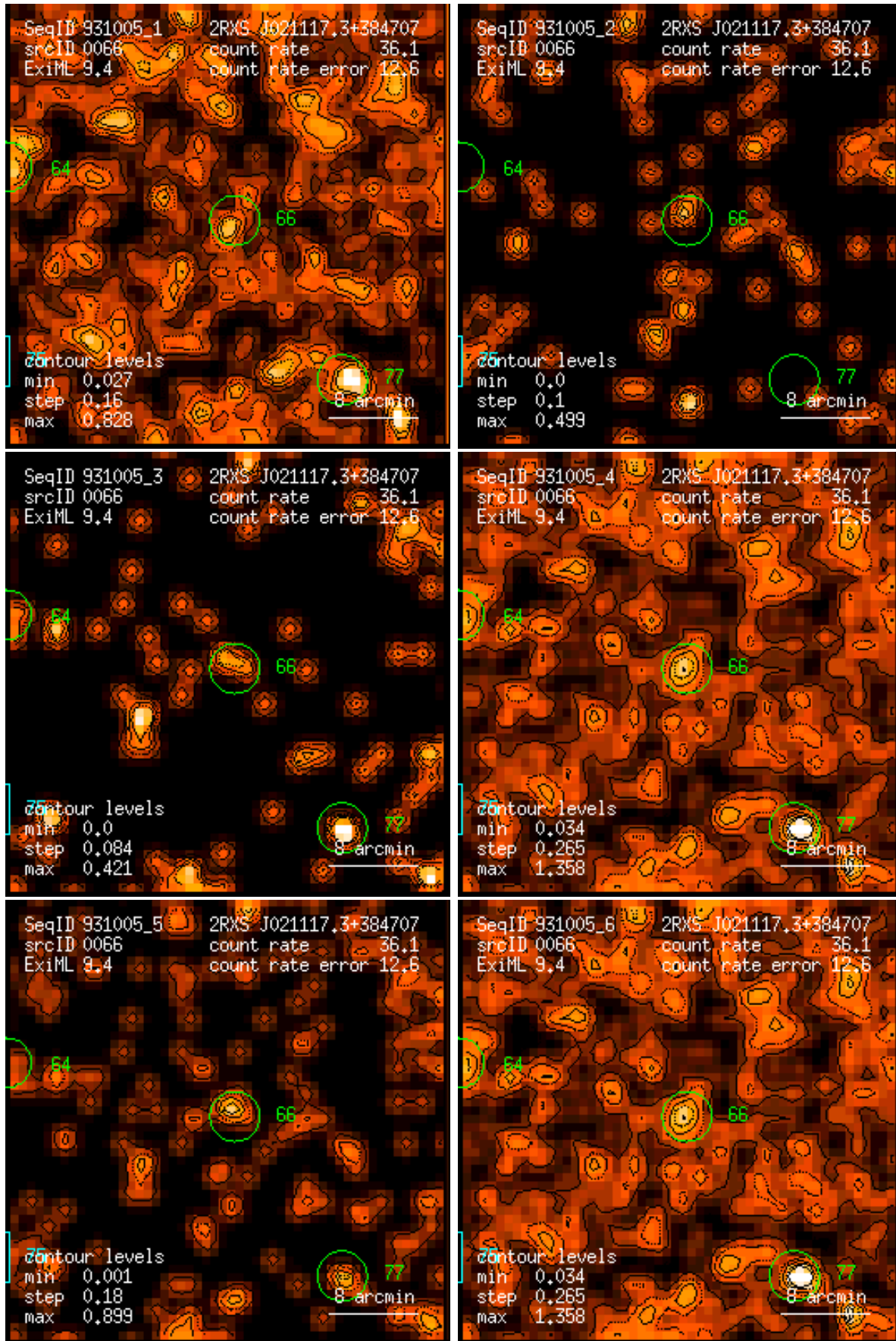
Figure 66: RASS 931005: detection 0066: band rate images, Gaussian filter: (1) PSPC channels 11 – 41, (2) 52 – 90, (3) 91 – 201, (4) 11 – 235, (5) 52 – 201, (6) 11 – 201. Broad band rates in counts/ks. Band rate contour levels in counts/ks/arcmin 2 .
