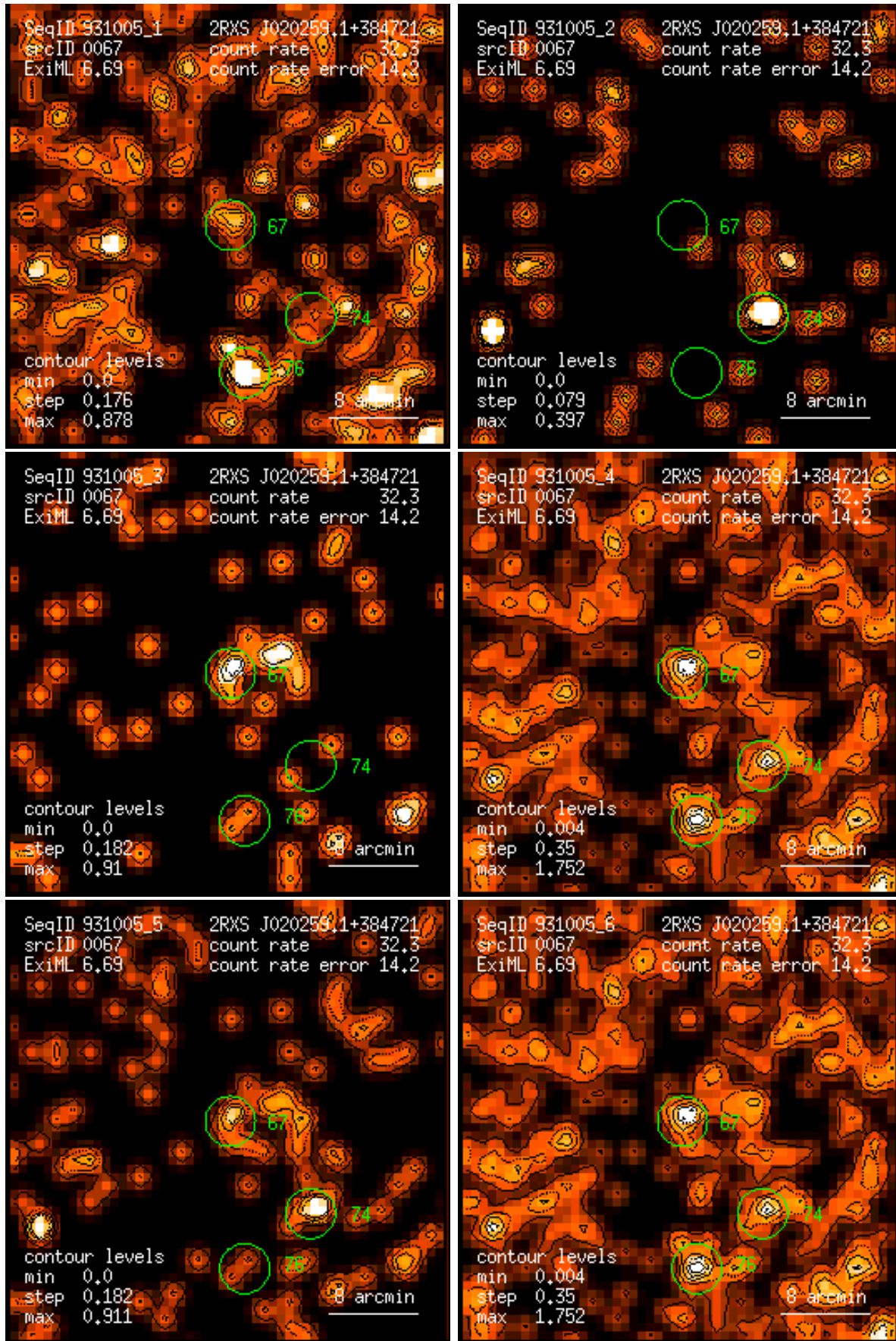
Figure 67: RASS 931005: detection 0067: band rate images, Gaussian filter: (1) PSPC channels 11 – 41, (2) 52 – 90, (3) 91 – 201, (4) 11 – 235, (5) 52 – 201, (6) 11 – 201. Broad band rates in counts/ks. Band rate contour levels in counts/ks/arcmin 2 .
