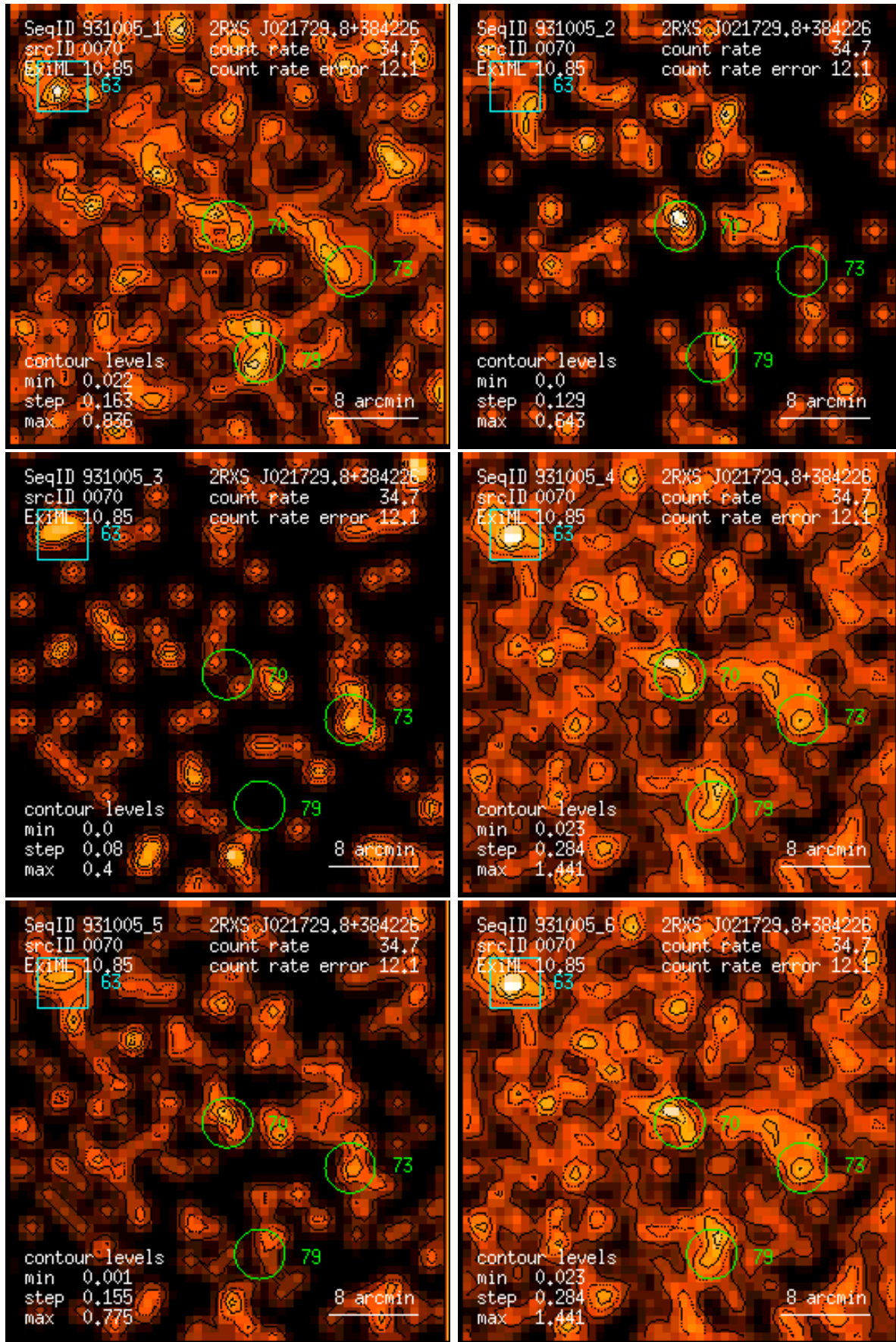
Figure 70: RASS 931005: detection 0070: band rate images, Gaussian filter: (1) PSPC channels 11 – 41, (2) 52 – 90, (3) 91 – 201, (4) 11 – 235, (5) 52 – 201, (6) 11 – 201. Broad band rates in counts/ks. Band rate contour levels in counts/ks/arcmin 2 .
