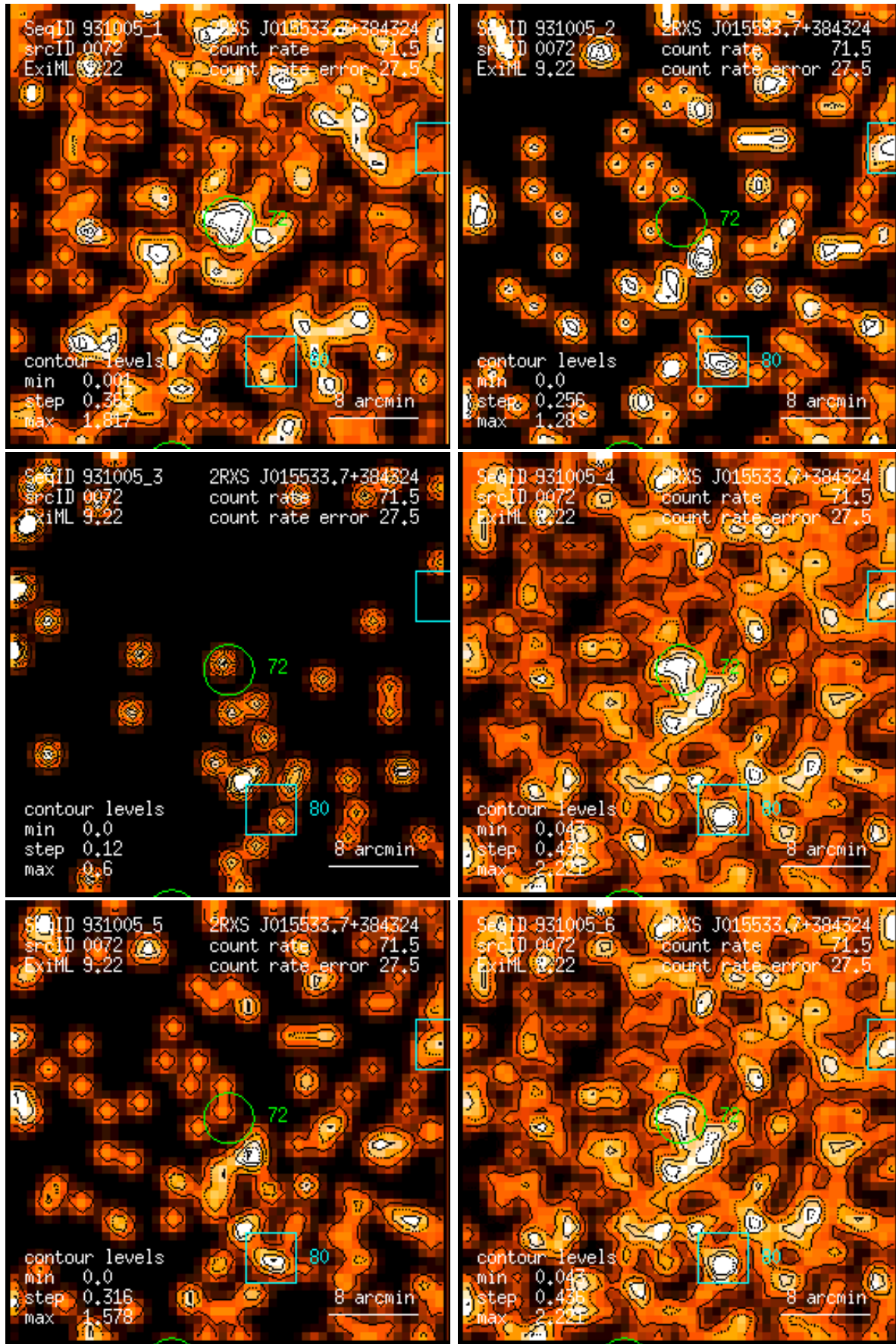
Figure 72: RASS 931005: detection 0072: band rate images, Gaussian filter: (1) PSPC channels 11 – 41, (2) 52 – 90, (3) 91 – 201, (4) 11 – 235, (5) 52 – 201, (6) 11 – 201. Broad band rates in counts/ks. Band rate contour levels in counts/ks/arcmin 2 .
