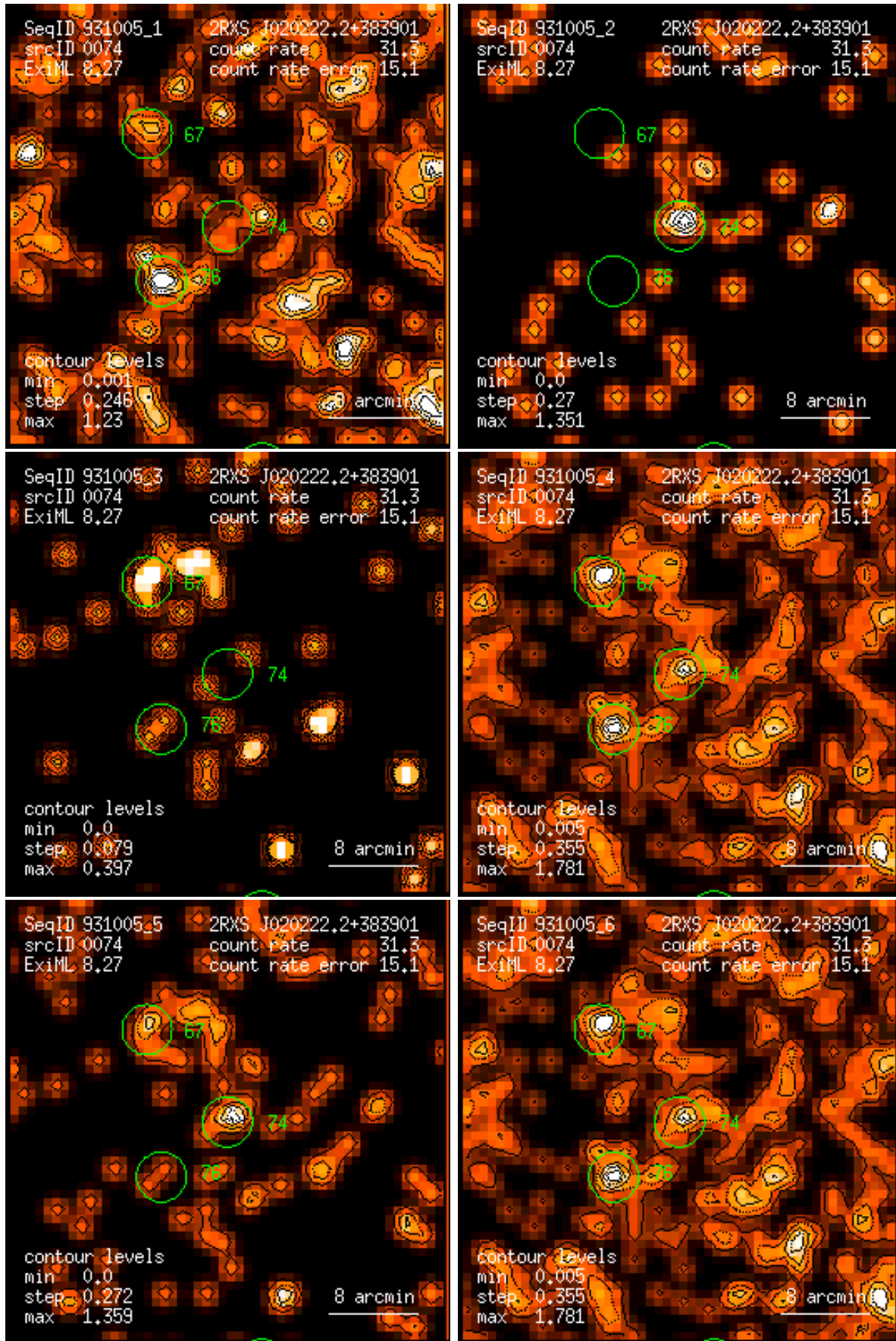
Figure 74: RASS 931005: detection 0074: band rate images, Gaussian filter: (1) PSPC channels 11 – 41, (2) 52 – 90, (3) 91 – 201, (4) 11 – 235, (5) 52 – 201, (6) 11 – 201. Broad band rates in counts/ks. Band rate contour levels in counts/ks/arcmin 2 .
