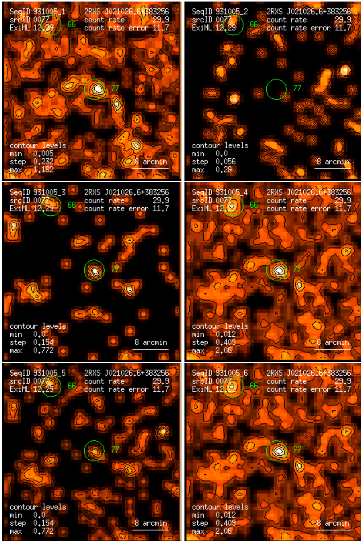
Figure 77: RASS 931005: detection 0077: band rate images, Gaussian filter: (1) PSPC channels 11 – 41, (2) 52 – 90, (3) 91 – 201, (4) 11 – 235, (5) 52 – 201, (6) 11 – 201. Broad band rates in counts/ks. Band rate contour levels in counts/ks/arcmin 2 .
