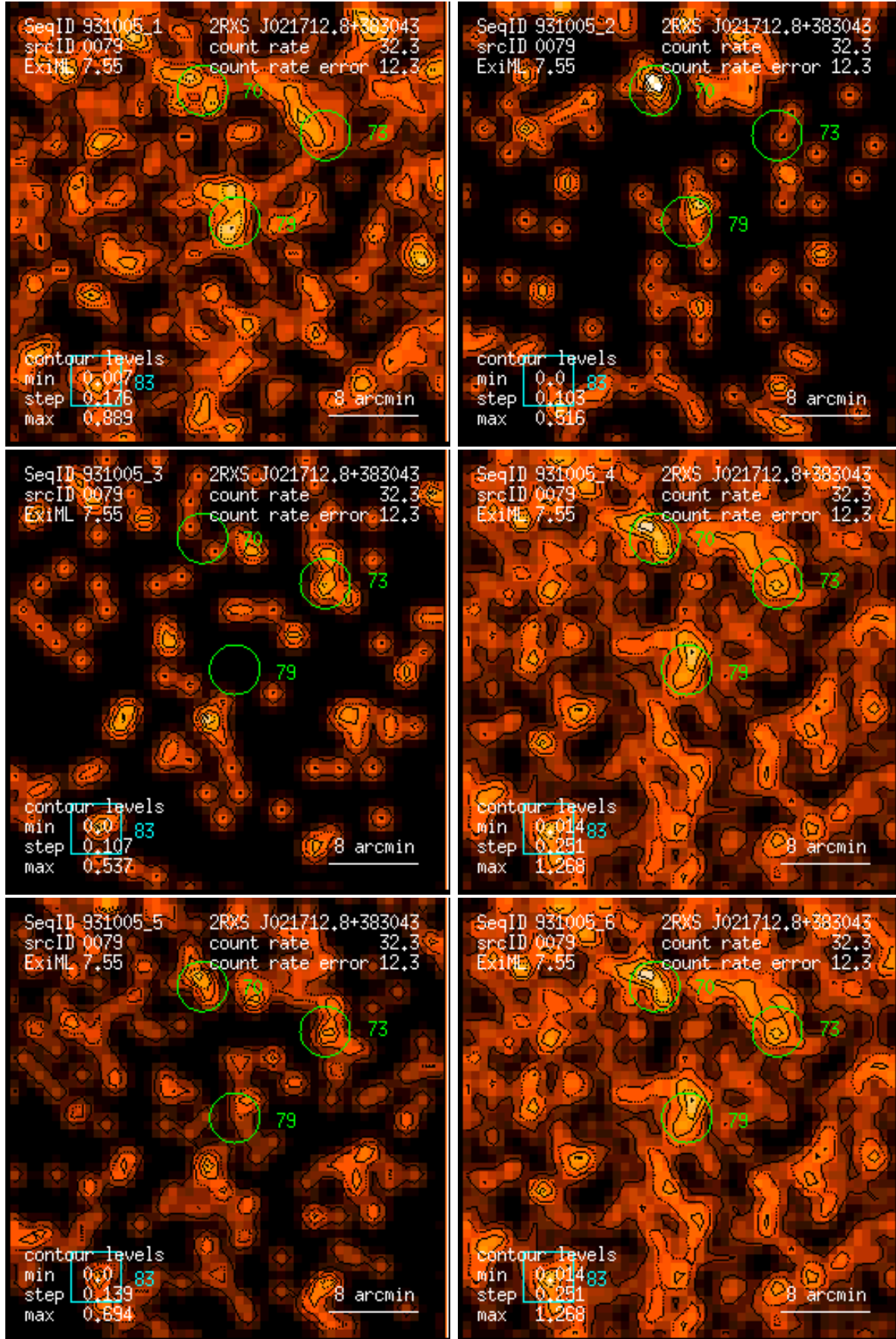
Figure 79: RASS 931005: detection 0079: band rate images, Gaussian filter: (1) PSPC channels 11 – 41, (2) 52 – 90, (3) 91 – 201, (4) 11 – 235, (5) 52 – 201, (6) 11 – 201. Broad band rates in counts/ks. Band rate contour levels in counts/ks/arcmin 2 .
