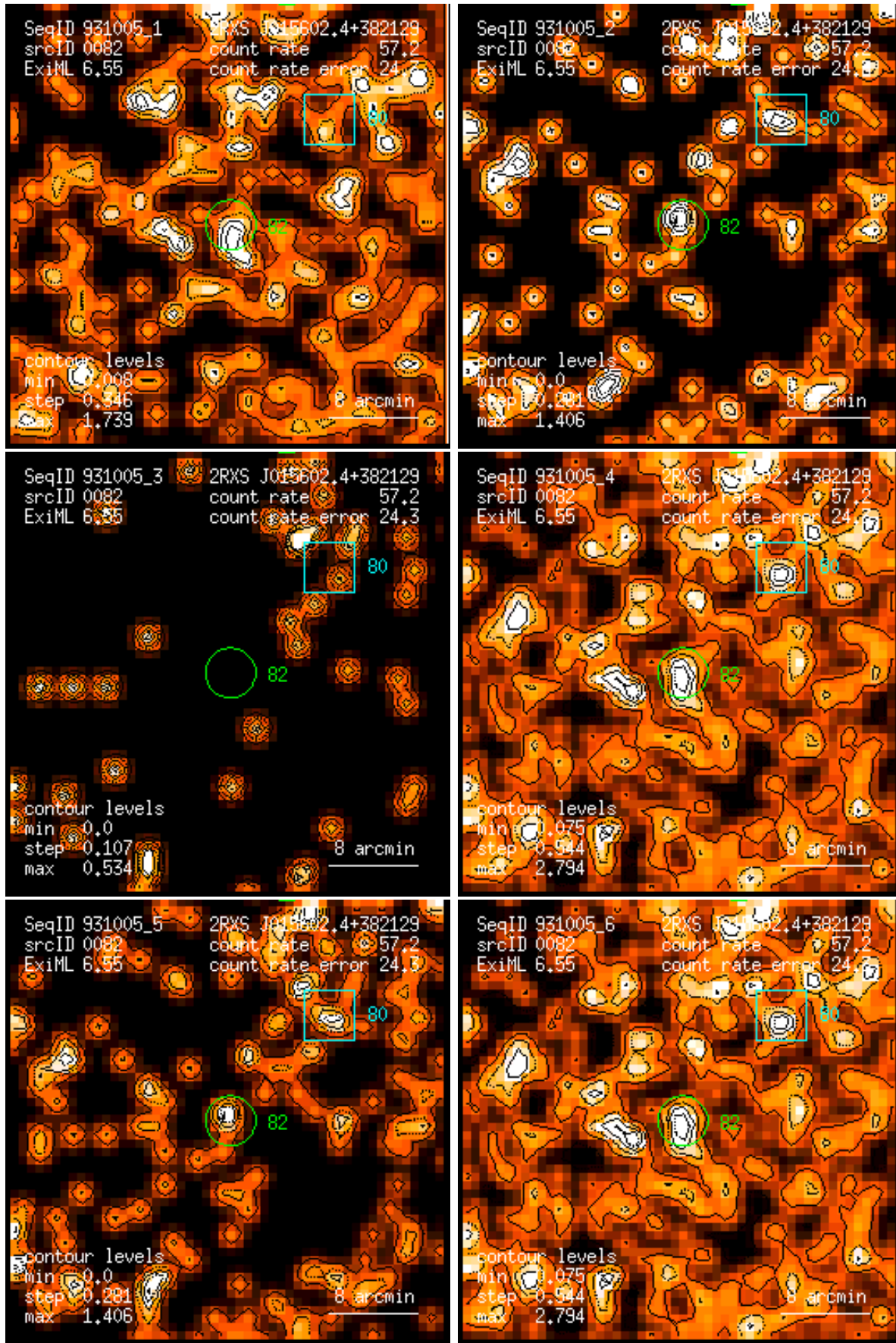
Figure 82: RASS 931005: detection 0082: band rate images, Gaussian filter: (1) PSPC channels 11 – 41, (2) 52 – 90, (3) 91 – 201, (4) 11 – 235, (5) 52 – 201, (6) 11 – 201. Broad band rates in counts/ks. Band rate contour levels in counts/ks/arcmin 2 .
