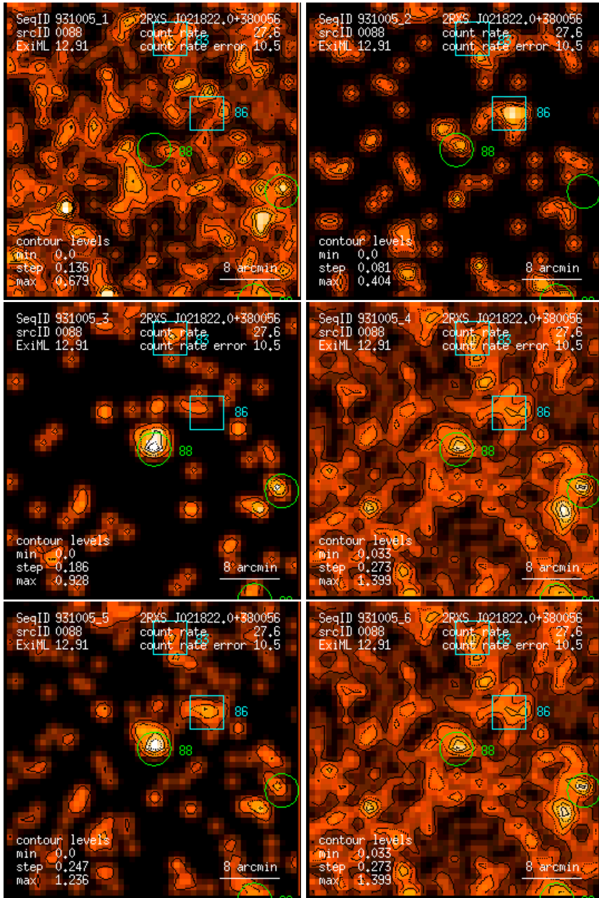
Figure 88: RASS 931005: detection 0088: band rate images, Gaussian filter: (1) PSPC channels 11 – 41, (2) 52 – 90, (3) 91 – 201, (4) 11 – 235, (5) 52 – 201, (6) 11 – 201. Broad band rates in counts/ks. Band rate contour levels in counts/ks/arcmin 2 .
