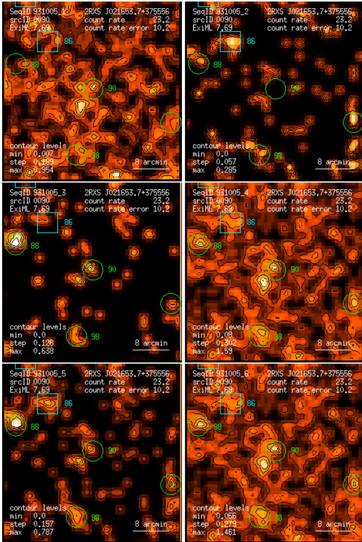
Figure 90: RASS 931005: detection 0090: band rate images, Gaussian filter: (1) PSPC channels 11 – 41, (2) 52 – 90, (3) 91 – 201, (4) 11 – 235, (5) 52 – 201, (6) 11 – 201. Broad band rates in counts/ks. Band rate contour levels in counts/ks/arcmin 2 .
