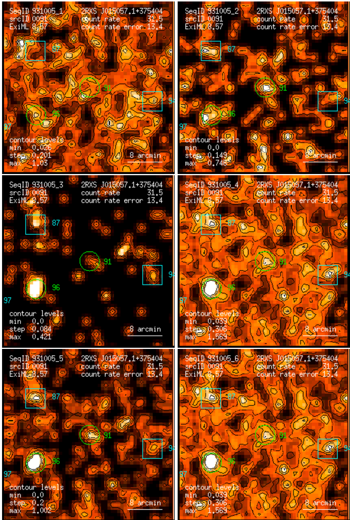
Figure 91: RASS 931005: detection 0091: band rate images, Gaussian filter: (1) PSPC channels 11 – 41, (2) 52 – 90, (3) 91 – 201, (4) 11 – 235, (5) 52 – 201, (6) 11 – 201. Broad band rates in counts/ks. Band rate contour levels in counts/ks/arcmin 2 .
