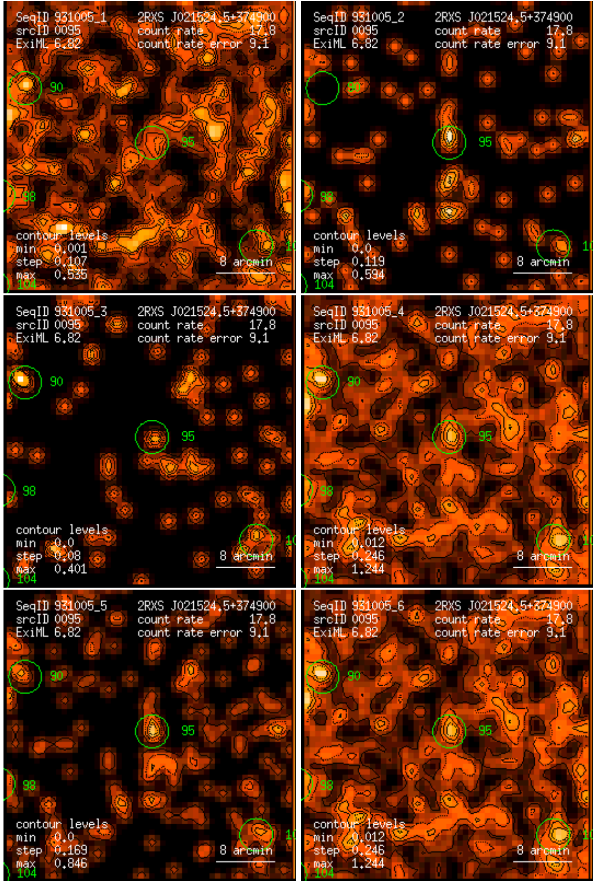
Figure 95: RASS 931005: detection 0095: band rate images, Gaussian filter: (1) PSPC channels 11 – 41, (2) 52 – 90, (3) 91 – 201, (4) 11 – 235, (5) 52 – 201, (6) 11 – 201. Broad band rates in counts/ks. Band rate contour levels in counts/ks/arcmin 2 .
