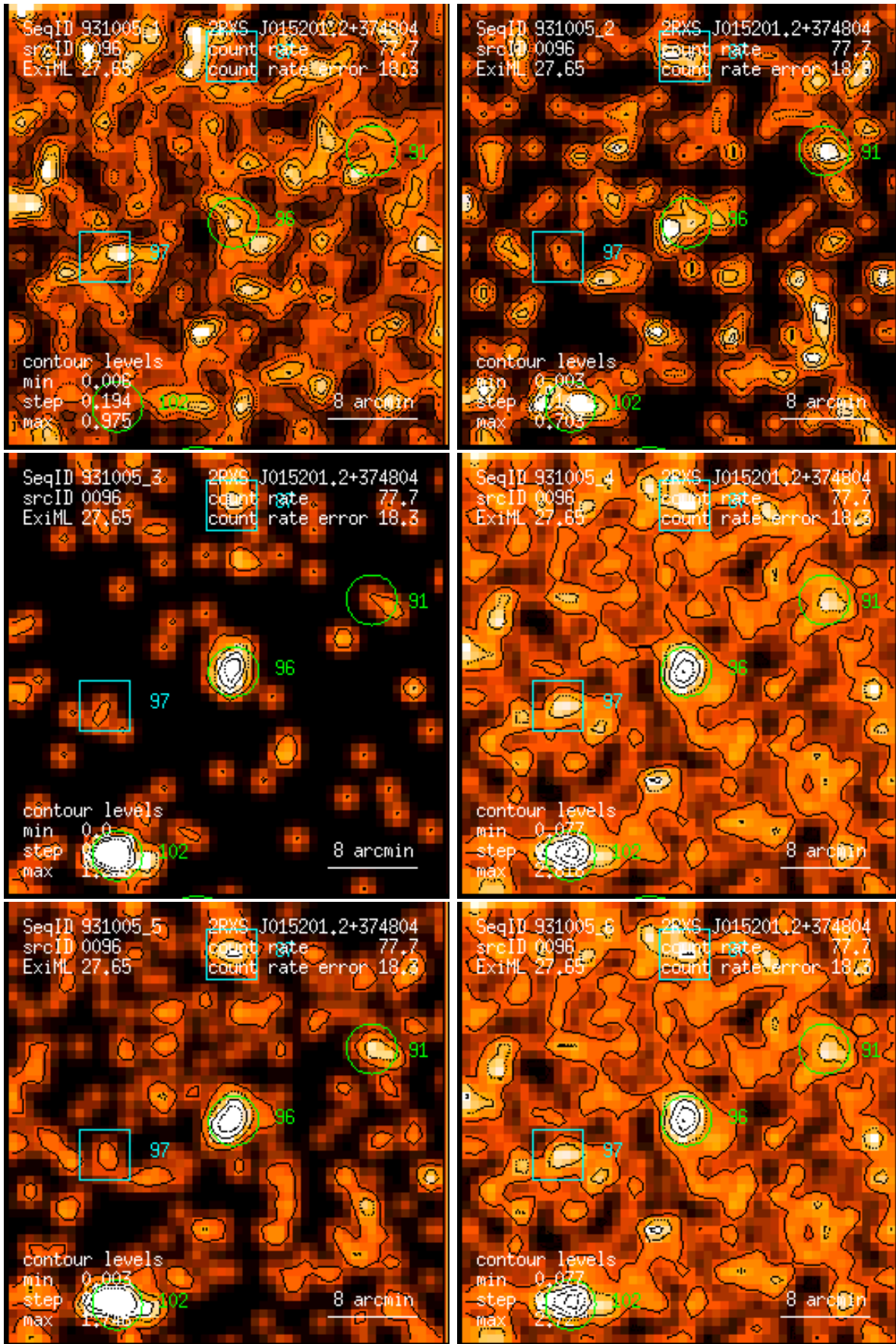
Figure 96: RASS 931005: detection 0096: band rate images, Gaussian filter: (1) PSPC channels 11 – 41, (2) 52 – 90, (3) 91 – 201, (4) 11 – 235, (5) 52 – 201, (6) 11 – 201. Broad band rates in counts/ks. Band rate contour levels in counts/ks/arcmin 2 .
