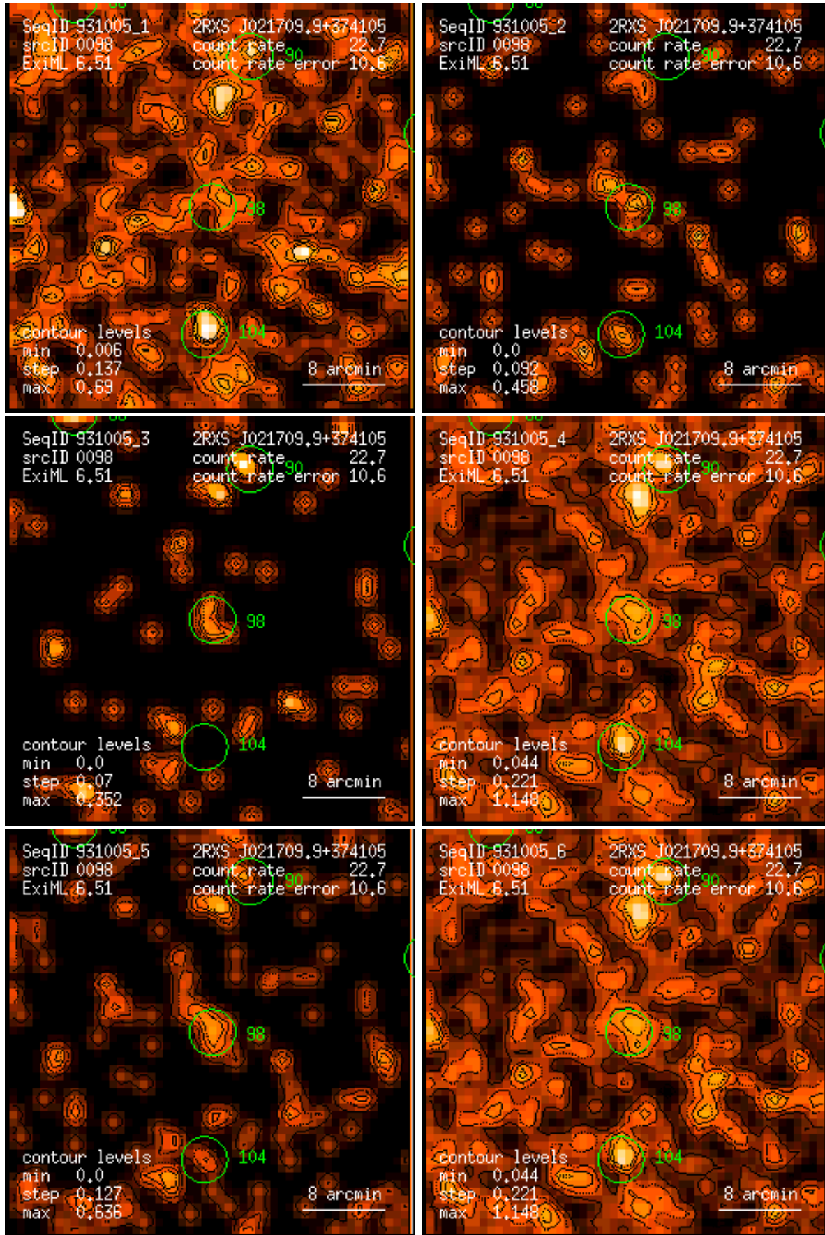
Figure 98: RASS 931005: detection 0098: band rate images, Gaussian filter: (1) PSPC channels 11 – 41, (2) 52 – 90, (3) 91 – 201, (4) 11 – 235, (5) 52 – 201, (6) 11 – 201. Broad band rates in counts/ks. Band rate contour levels in counts/ks/arcmin 2 .
