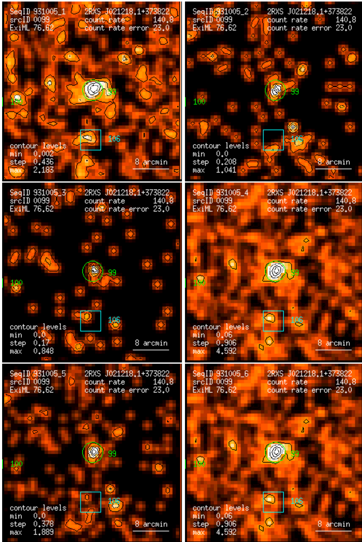
Figure 99: RASS 931005: detection 0099: band rate images, Gaussian filter: (1) PSPC channels 11 – 41, (2) 52 – 90, (3) 91 – 201, (4) 11 – 235, (5) 52 – 201, (6) 11 – 201. Broad band rates in counts/ks. Band rate contour levels in counts/ks/arcmin 2 .
