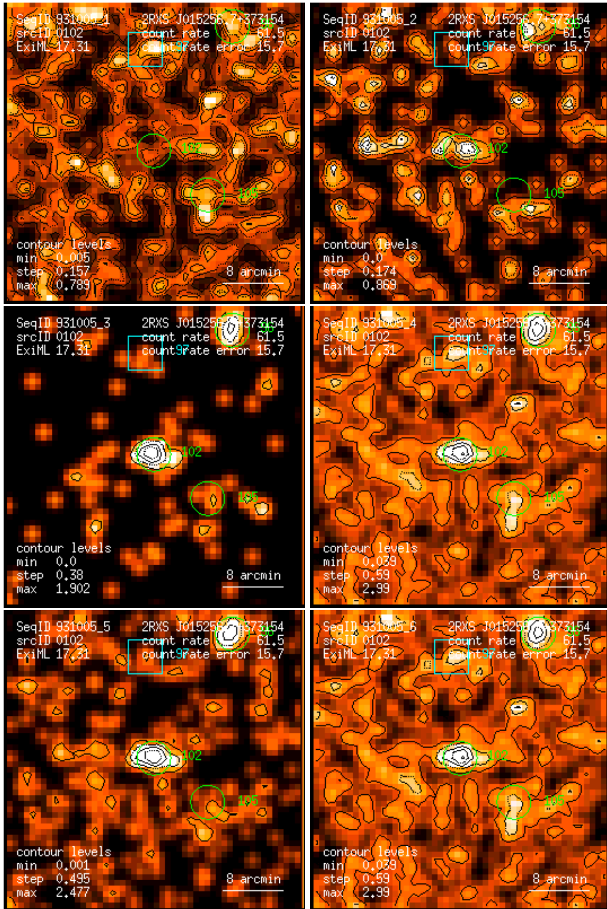
Figure 102: RASS 931005: detection 0102: band rate images, Gaussian filter: (1) PSPC channels 11 – 41, (2) 52 – 90, (3) 91 – 201, (4) 11 – 235, (5) 52 – 201, (6) 11 – 201. Broad band rates in counts/ks. Band rate contour levels in counts/ks/arcmin 2 .
