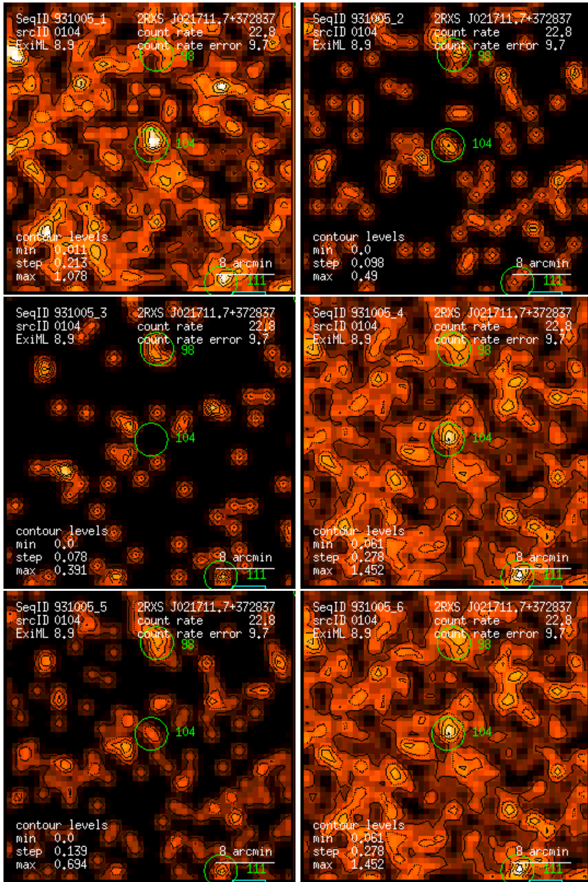
Figure 104: RASS 931005: detection 0104: band rate images, Gaussian filter: (1) PSPC channels 11 – 41, (2) 52 – 90, (3) 91 – 201, (4) 11 – 235, (5) 52 – 201, (6) 11 – 201. Broad band rates in counts/ks. Band rate contour levels in counts/ks/arcmin 2 .
