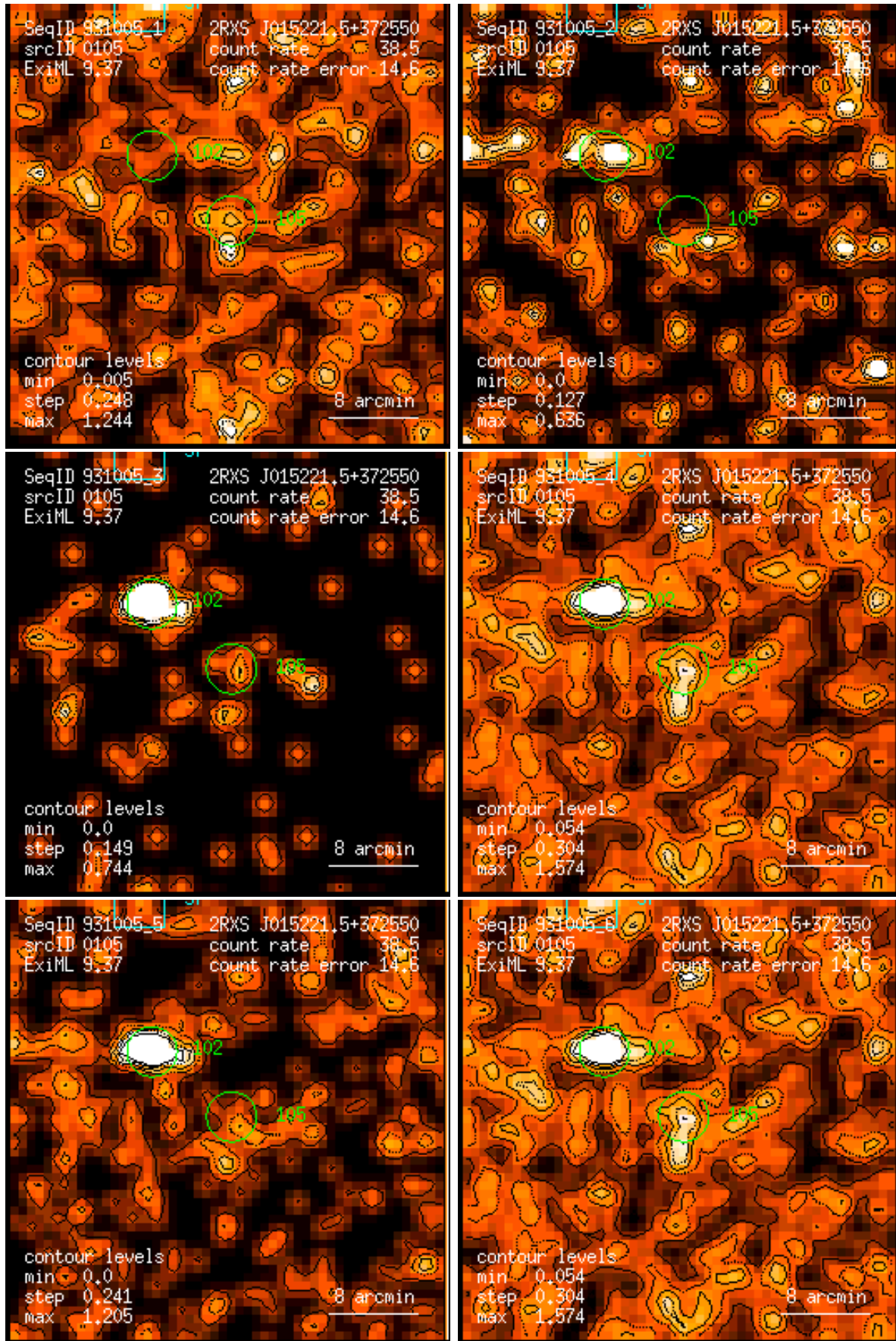
Figure 105: RASS 931005: detection 0105: band rate images, Gaussian filter: (1) PSPC channels 11 – 41, (2) 52 – 90, (3) 91 – 201, (4) 11 – 235, (5) 52 – 201, (6) 11 – 201. Broad band rates in counts/ks. Band rate contour levels in counts/ks/arcmin 2 .
