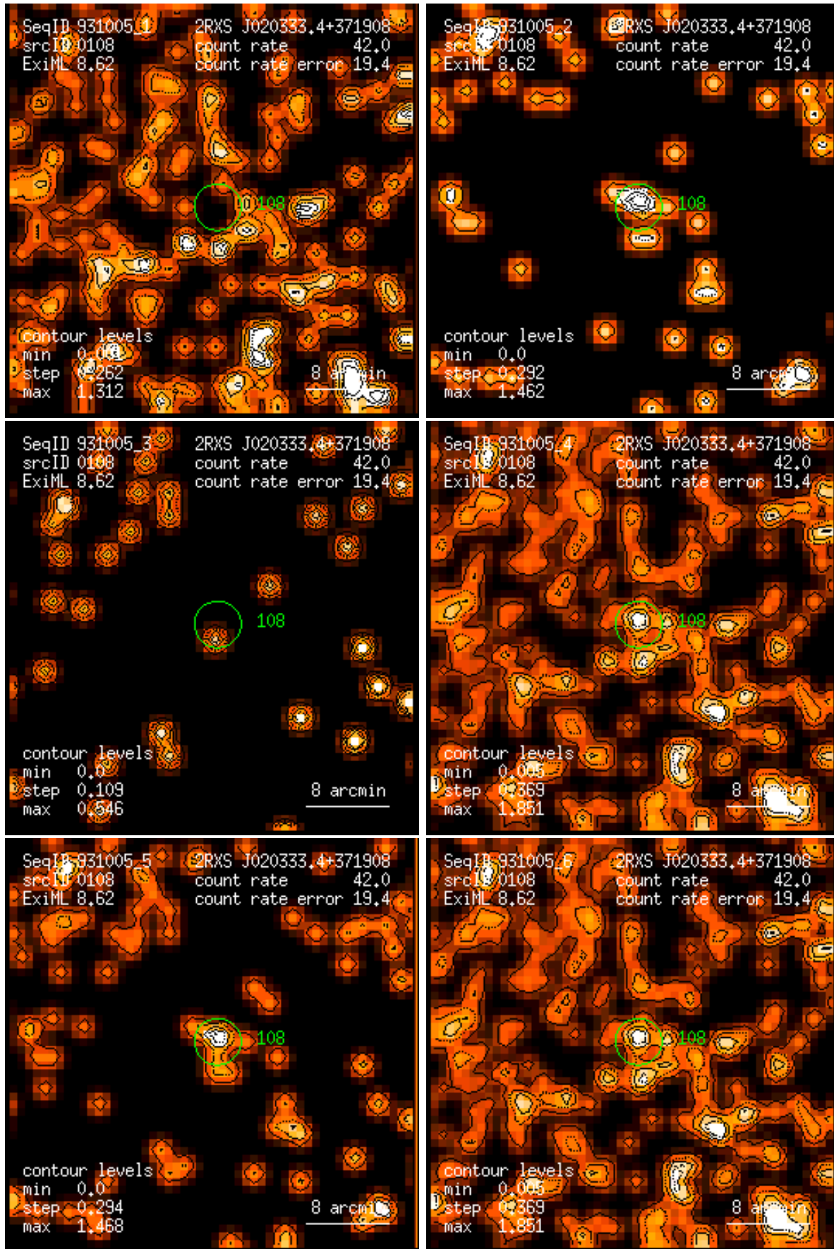
Figure 108: RASS 931005: detection 0108: band rate images, Gaussian filter: (1) PSPC channels 11 – 41, (2) 52 – 90, (3) 91 – 201, (4) 11 – 235, (5) 52 – 201, (6) 11 – 201. Broad band rates in counts/ks. Band rate contour levels in counts/ks/arcmin 2 .
