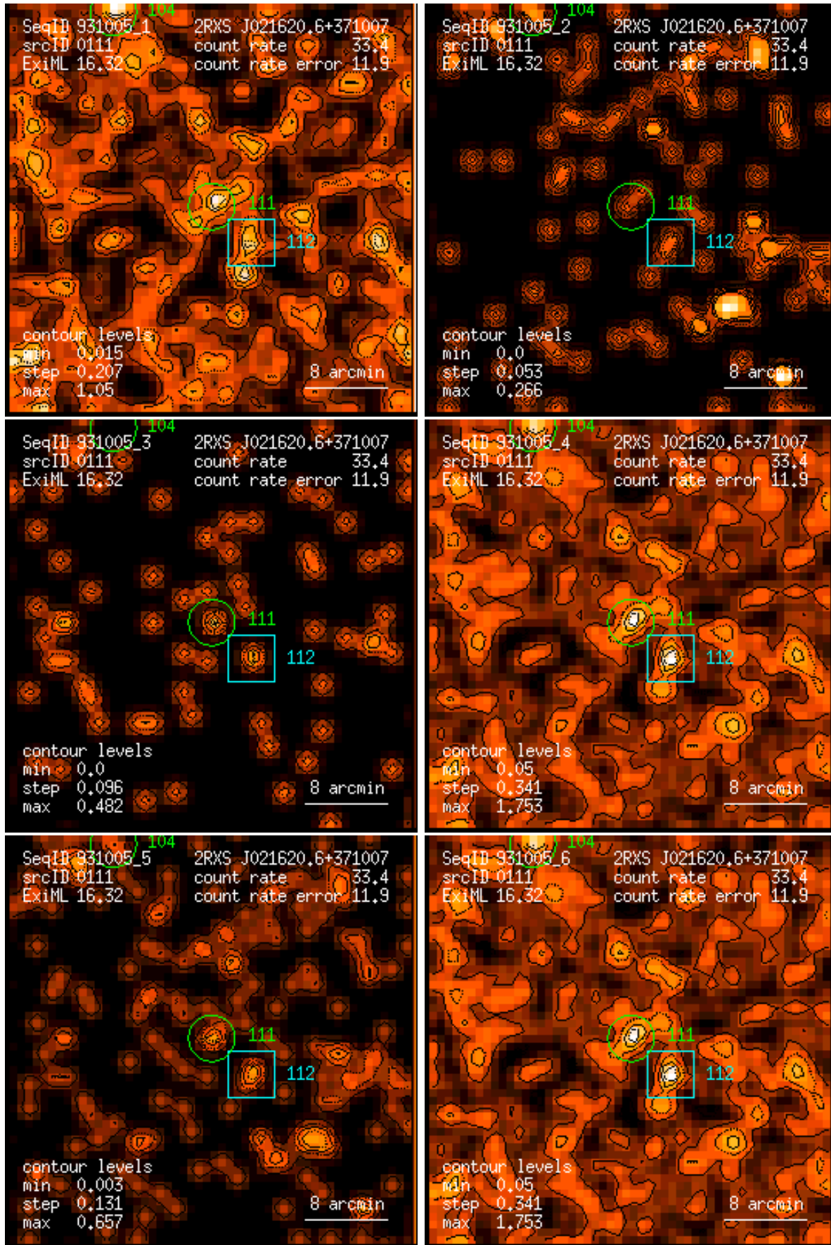
Figure 111: RASS 931005: detection 0111: band rate images, Gaussian filter: (1) PSPC channels 11 – 41, (2) 52 – 90, (3) 91 – 201, (4) 11 – 235, (5) 52 – 201, (6) 11 – 201. Broad band rates in counts/ks. Band rate contour levels in counts/ks/arcmin 2 .
