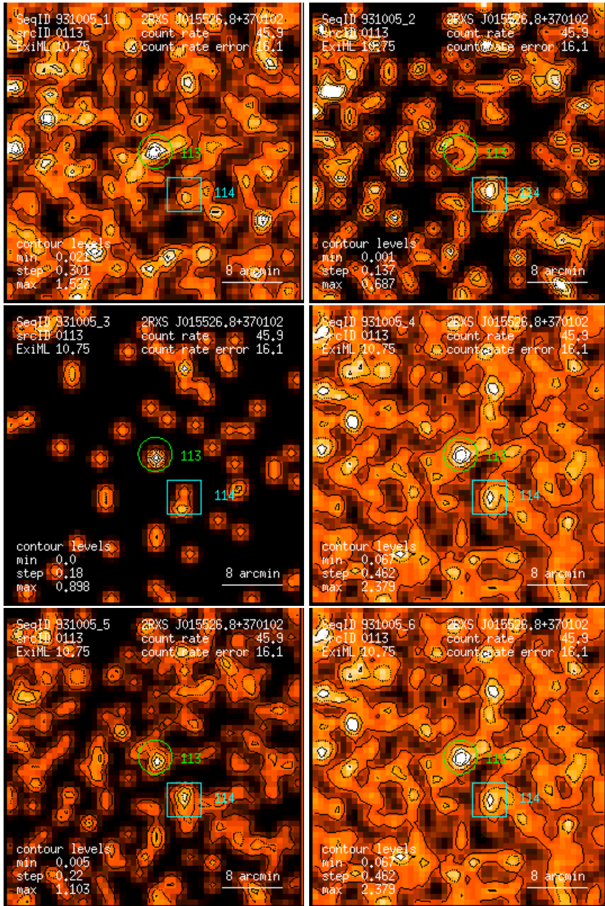
Figure 113: RASS 931005: detection 0113: band rate images, Gaussian filter: (1) PSPC channels 11 – 41, (2) 52 – 90, (3) 91 – 201, (4) 11 – 235, (5) 52 – 201, (6) 11 – 201. Broad band rates in counts/ks. Band rate contour levels in counts/ks/arcmin 2 .
