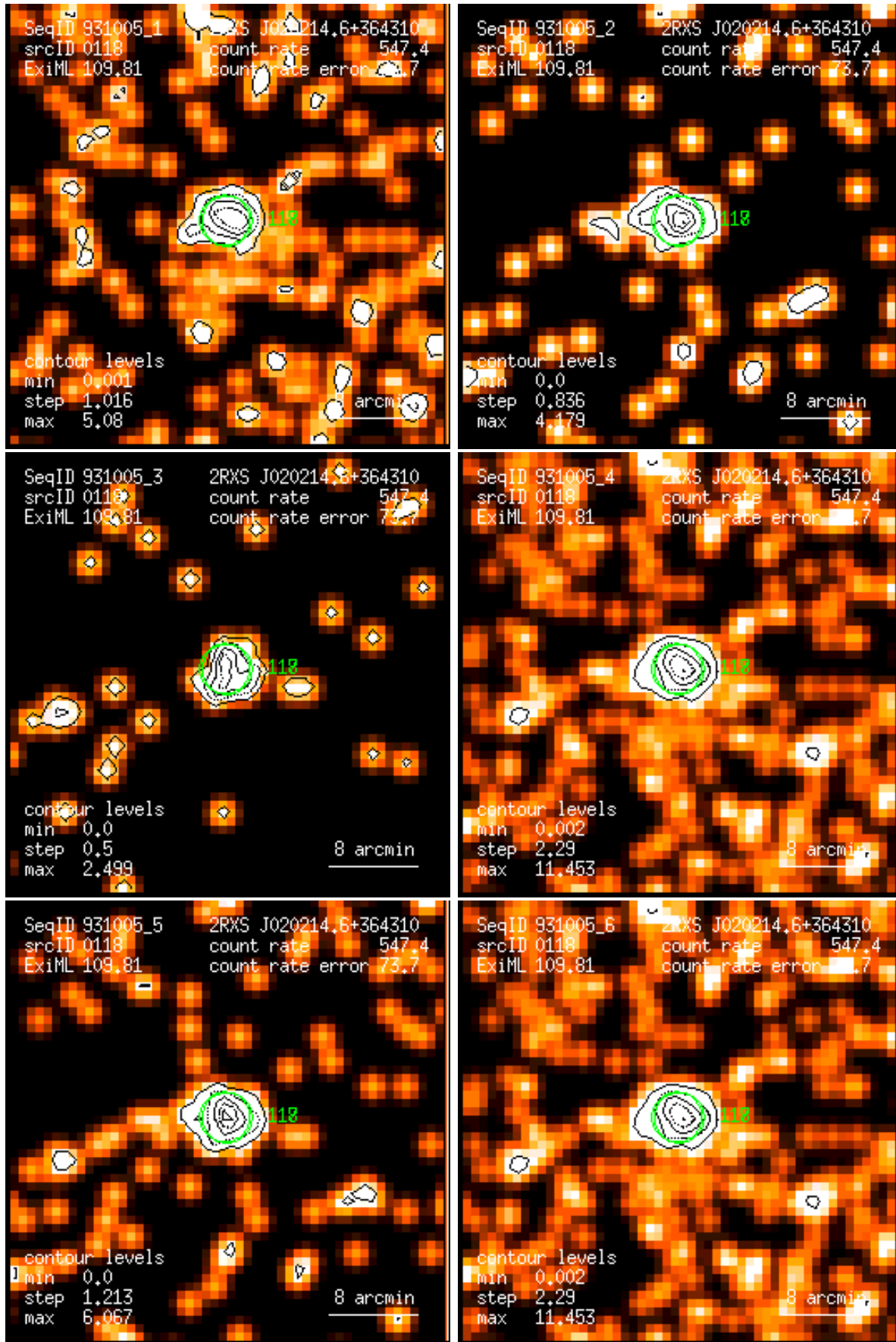
Figure 118: RASS 931005: detection 0118: band rate images, Gaussian filter: (1) PSPC channels 11 – 41, (2) 52 – 90, (3) 91 – 201, (4) 11 – 235, (5) 52 – 201, (6) 11 – 201. Broad band rates in counts/ks. Band rate contour levels in counts/ks/arcmin 2 .
