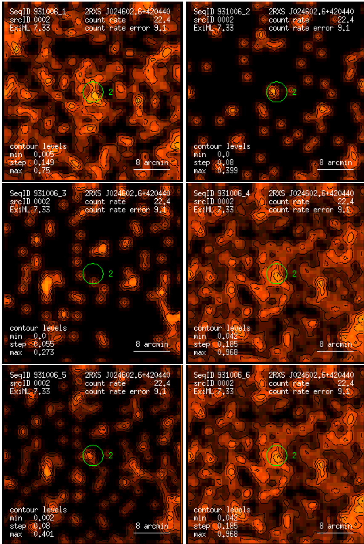
Figure 2: RASS 931006: detection 0002: band rate images, Gaussian filter: (1) PSPC channels 11 – 41, (2) 52 – 90, (3) 91 – 201, (4) 11 – 235, (5) 52 – 201, (6) 11 – 201. Broad band rates in counts/ks. Band rate contour levels in counts/ks/arcmin 2 .
