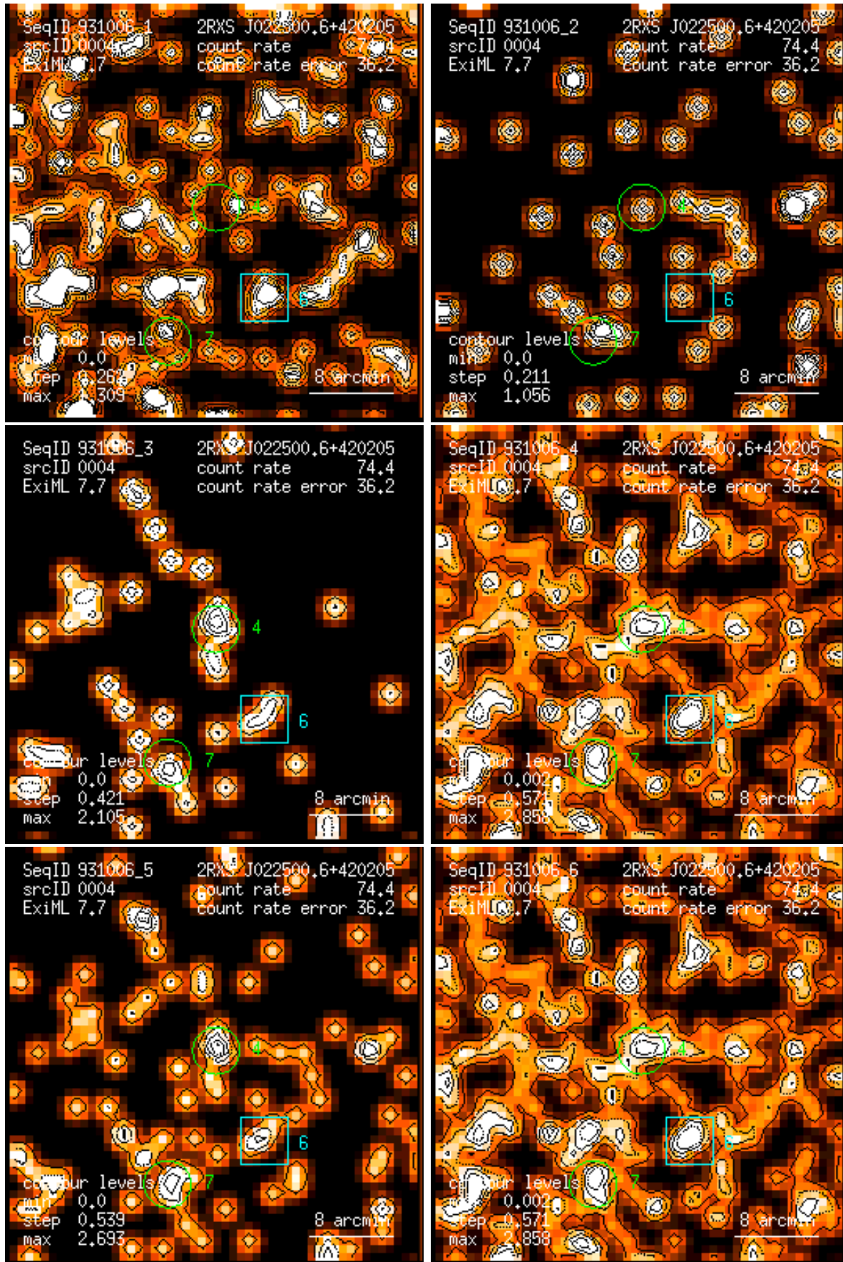
Figure 4: RASS 931006: detection 0004: band rate images, Gaussian filter: (1) PSPC channels 11 – 41, (2) 52 – 90, (3) 91 – 201, (4) 11 – 235, (5) 52 – 201, (6) 11 – 201. Broad band rates in counts/ks. Band rate contour levels in counts/ks/arcmin 2 .
