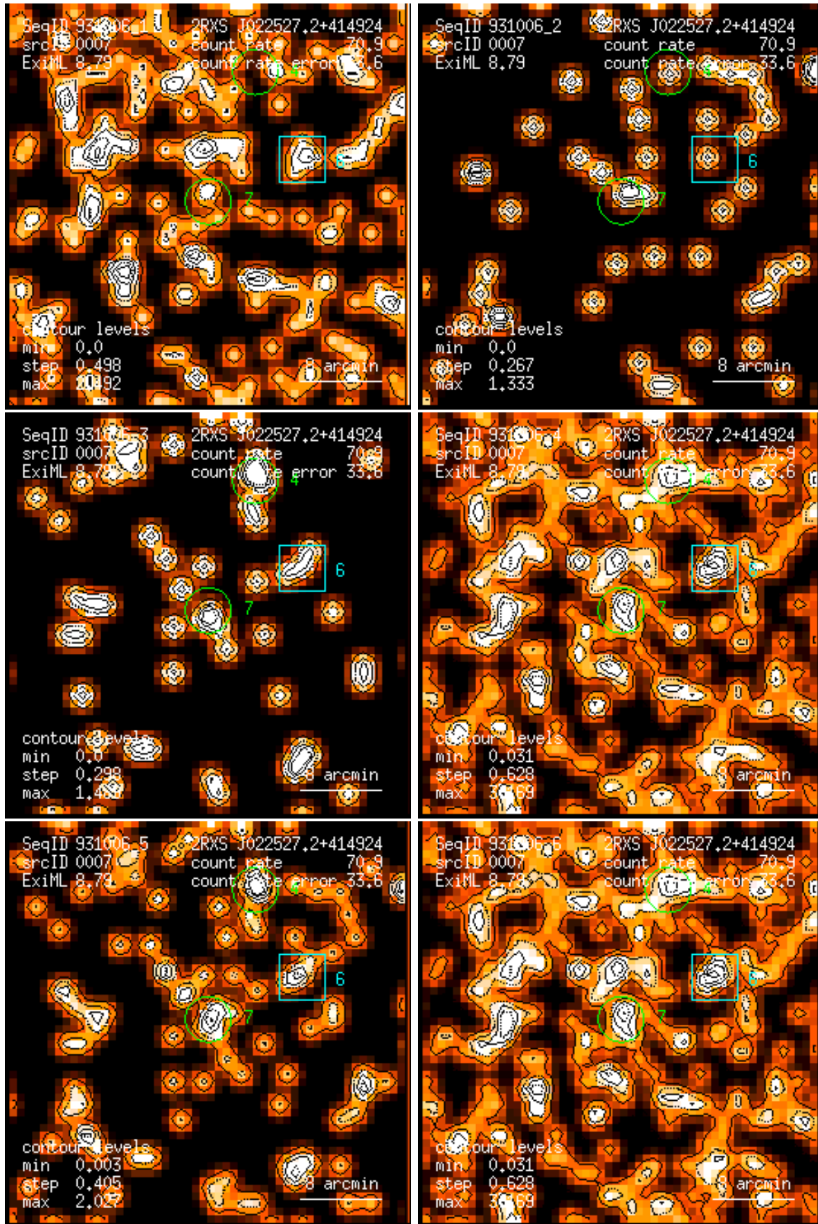
Figure 7: RASS 931006: detection 0007: band rate images, Gaussian filter: (1) PSPC channels 11 – 41, (2) 52 – 90, (3) 91 – 201, (4) 11 – 235, (5) 52 – 201, (6) 11 – 201. Broad band rates in counts/ks. Band rate contour levels in counts/ks/arcmin 2 .
