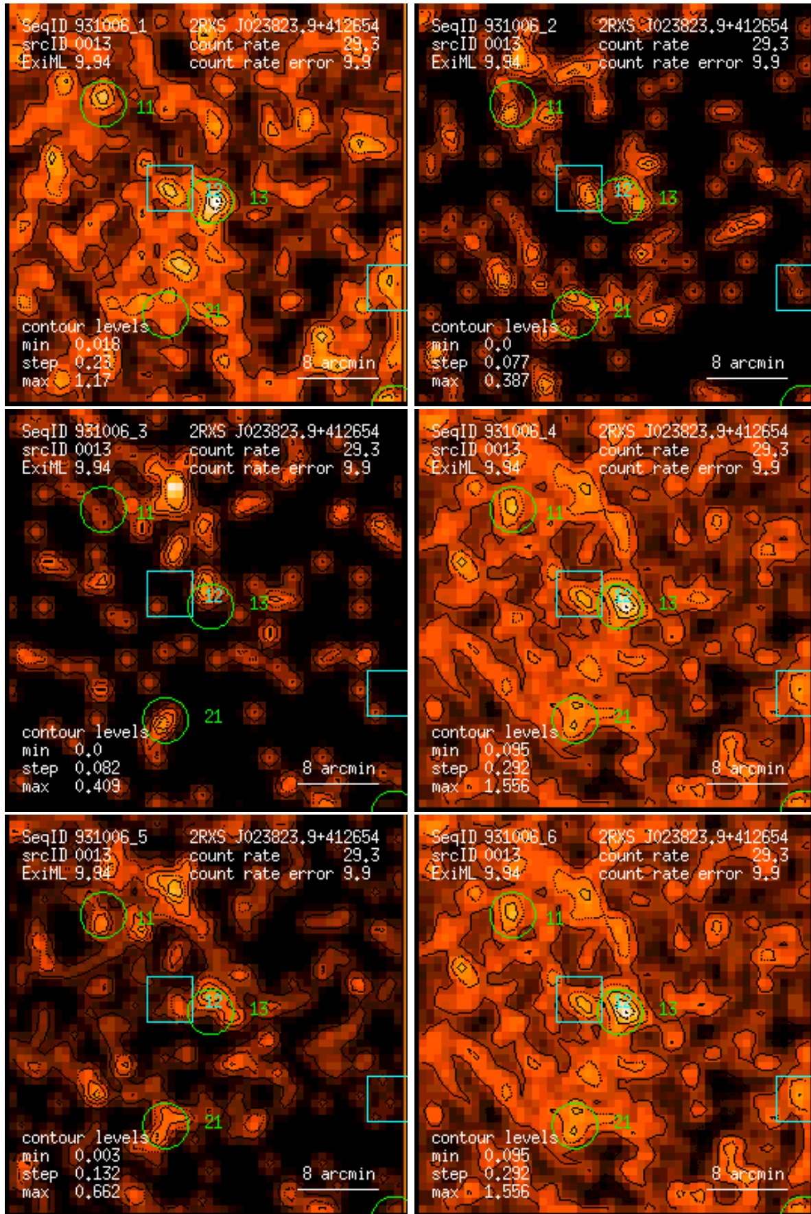
Figure 13: RASS 931006: detection 0013: band rate images, Gaussian filter: (1) PSPC channels 11 – 41, (2) 52 – 90, (3) 91 – 201, (4) 11 – 235, (5) 52 – 201, (6) 11 – 201. Broad band rates in counts/ks. Band rate contour levels in counts/ks/arcmin 2 .
