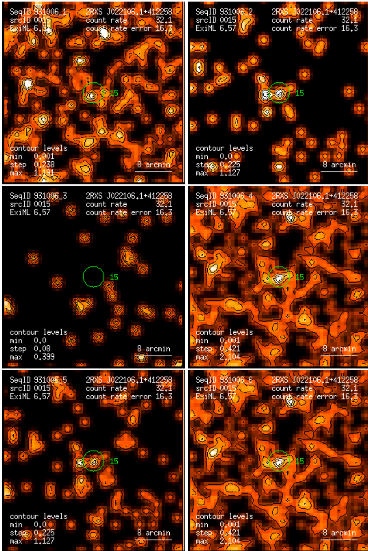
Figure 15: RASS 931006: detection 0015: band rate images, Gaussian filter: (1) PSPC channels 11 – 41, (2) 52 – 90, (3) 91 – 201, (4) 11 – 235, (5) 52 – 201, (6) 11 – 201. Broad band rates in counts/ks. Band rate contour levels in counts/ks/arcmin 2 .
