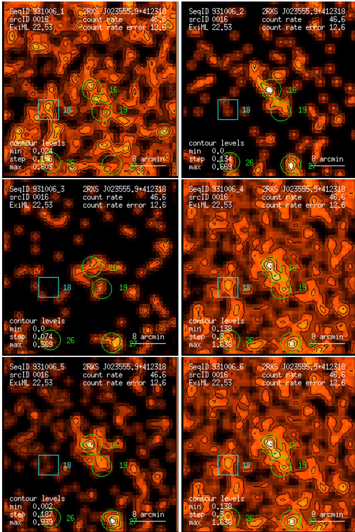
Figure 16: RASS 931006: detection 0016: band rate images, Gaussian filter: (1) PSPC channels 11 – 41, (2) 52 – 90, (3) 91 – 201, (4) 11 – 235, (5) 52 – 201, (6) 11 – 201. Broad band rates in counts/ks. Band rate contour levels in counts/ks/arcmin 2 .
