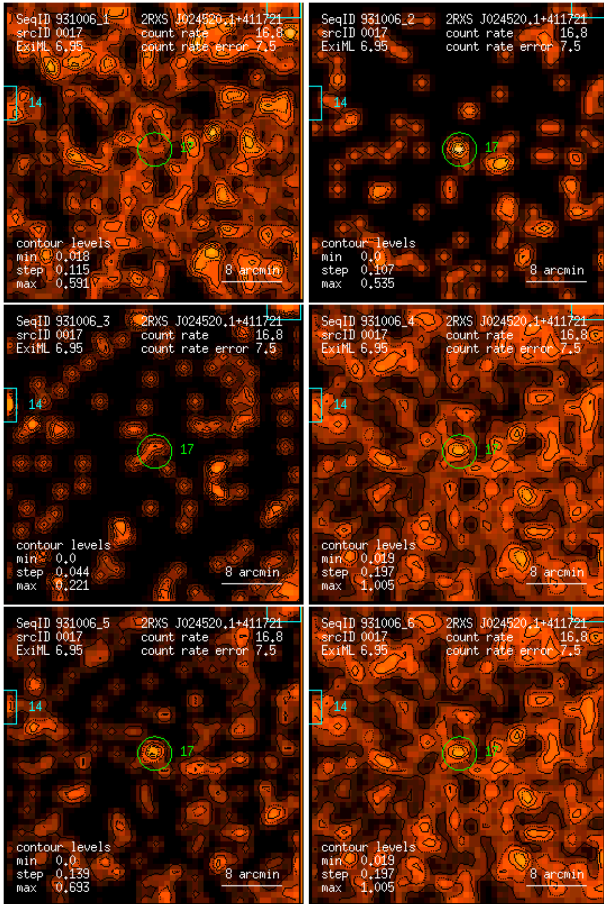
Figure 17: RASS 931006: detection 0017: band rate images, Gaussian filter: (1) PSPC channels 11 – 41, (2) 52 – 90, (3) 91 – 201, (4) 11 – 235, (5) 52 – 201, (6) 11 – 201. Broad band rates in counts/ks. Band rate contour levels in counts/ks/arcmin 2 .
