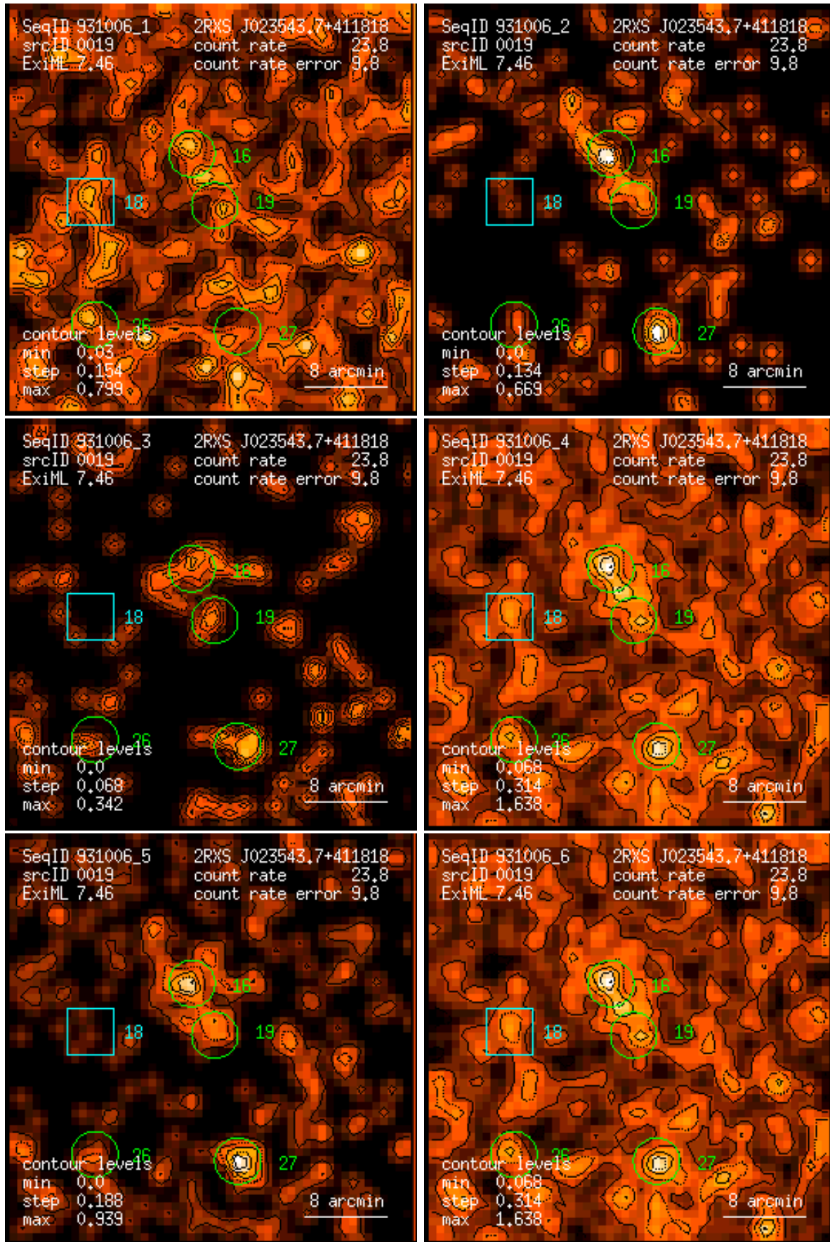
Figure 19: RASS 931006: detection 0019: band rate images, Gaussian filter: (1) PSPC channels 11 – 41, (2) 52 – 90, (3) 91 – 201, (4) 11 – 235, (5) 52 – 201, (6) 11 – 201. Broad band rates in counts/ks. Band rate contour levels in counts/ks/arcmin 2 .
