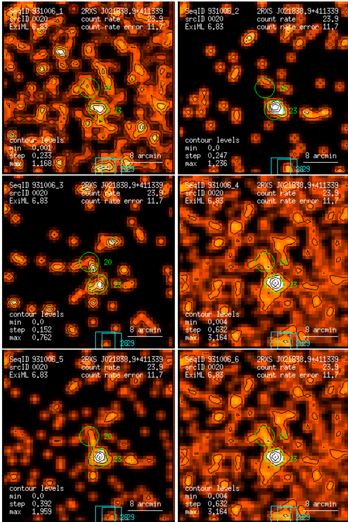
Figure 20: RASS 931006: detection 0020: band rate images, Gaussian filter: (1) PSPC channels 11 – 41, (2) 52 – 90, (3) 91 – 201, (4) 11 – 235, (5) 52 – 201, (6) 11 – 201. Broad band rates in counts/ks. Band rate contour levels in counts/ks/arcmin 2 .
