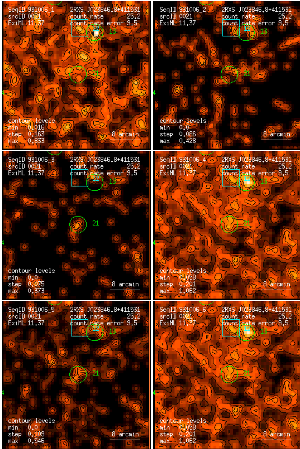
Figure 21: RASS 931006: detection 0021: band rate images, Gaussian filter: (1) PSPC channels 11 – 41, (2) 52 – 90, (3) 91 – 201, (4) 11 – 235, (5) 52 – 201, (6) 11 – 201. Broad band rates in counts/ks. Band rate contour levels in counts/ks/arcmin 2 .
