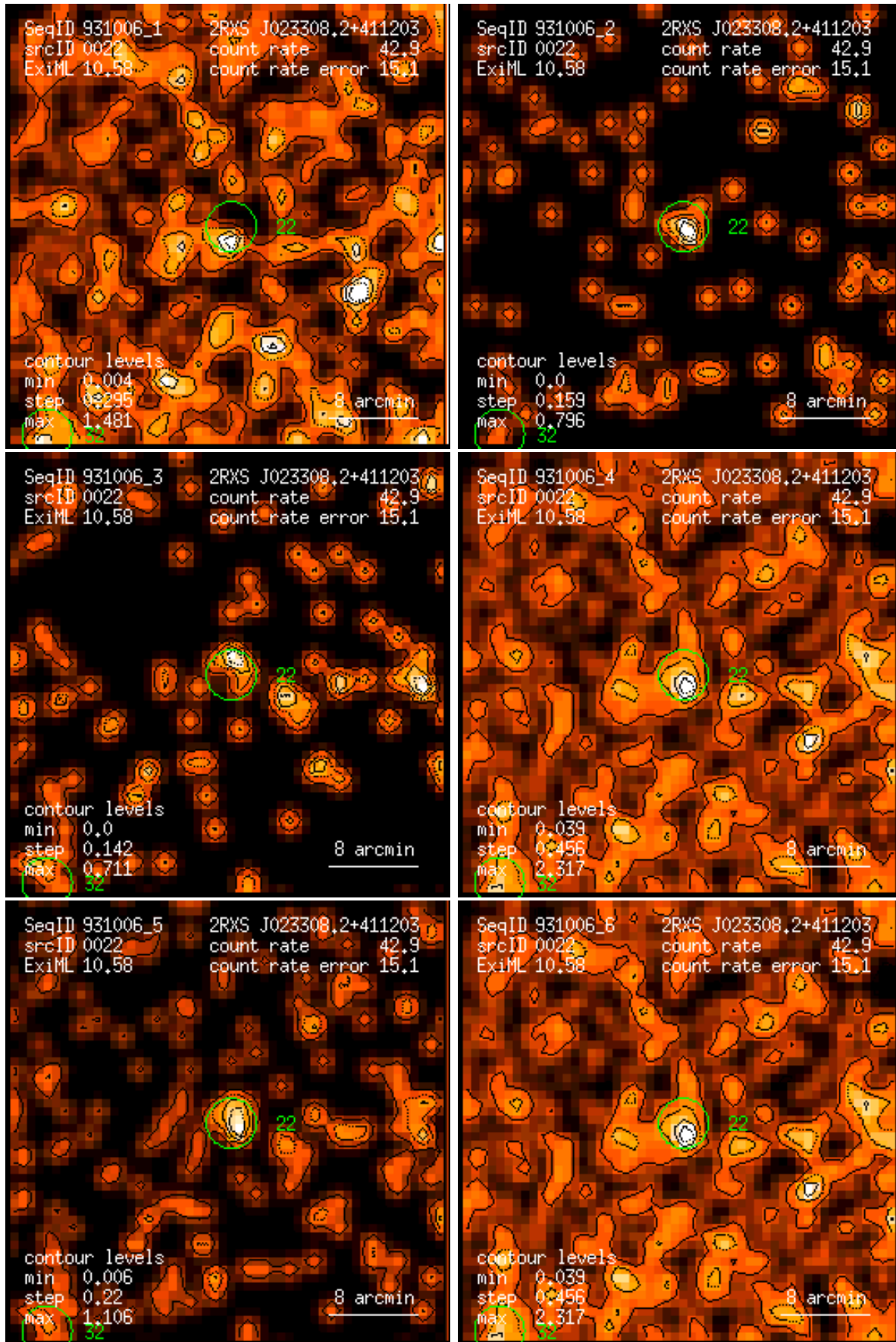
Figure 22: RASS 931006: detection 0022: band rate images, Gaussian filter: (1) PSPC channels 11 – 41, (2) 52 – 90, (3) 91 – 201, (4) 11 – 235, (5) 52 – 201, (6) 11 – 201. Broad band rates in counts/ks. Band rate contour levels in counts/ks/arcmin 2 .
