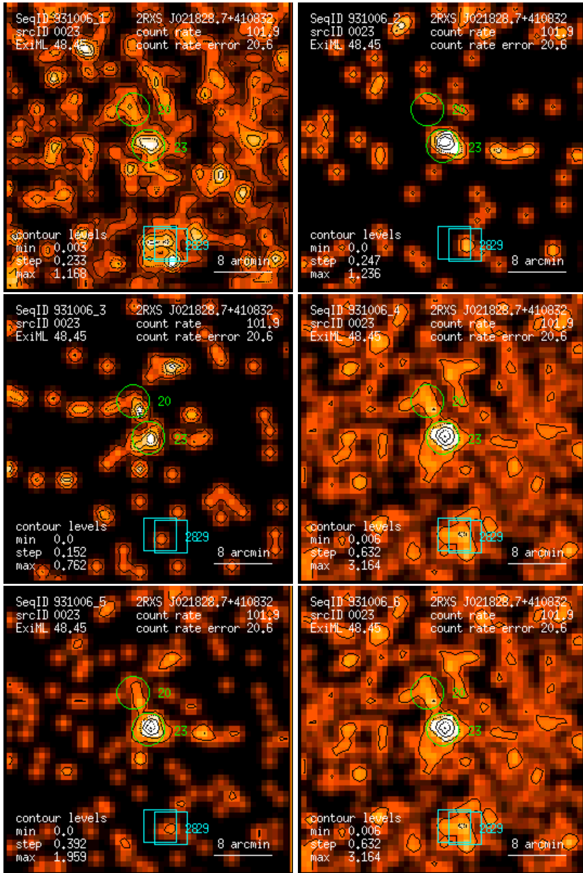
Figure 23: RASS 931006: detection 0023: band rate images, Gaussian filter: (1) PSPC channels 11 – 41, (2) 52 – 90, (3) 91 – 201, (4) 11 – 235, (5) 52 – 201, (6) 11 – 201. Broad band rates in counts/ks. Band rate contour levels in counts/ks/arcmin 2 .
