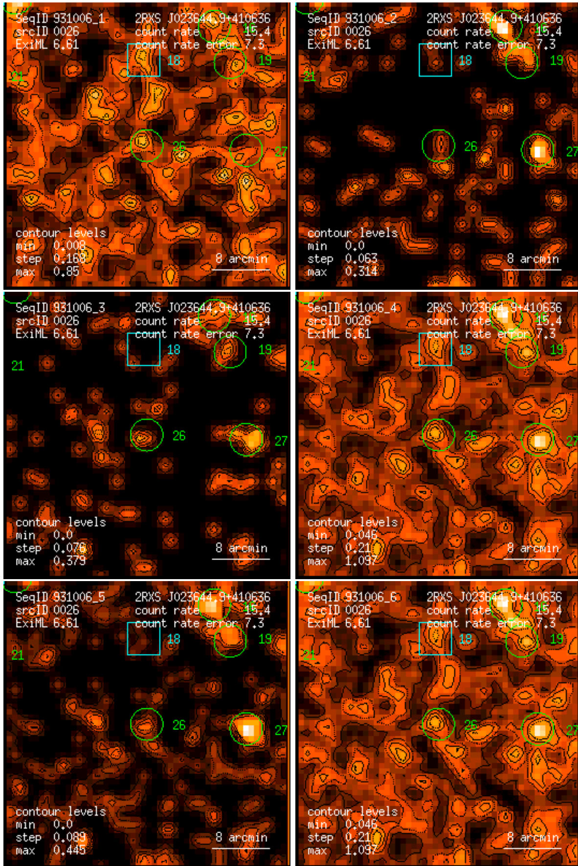
Figure 26: RASS 931006: detection 0026: band rate images, Gaussian filter: (1) PSPC channels 11 – 41, (2) 52 – 90, (3) 91 – 201, (4) 11 – 235, (5) 52 – 201, (6) 11 – 201. Broad band rates in counts/ks. Band rate contour levels in counts/ks/arcmin 2 .
