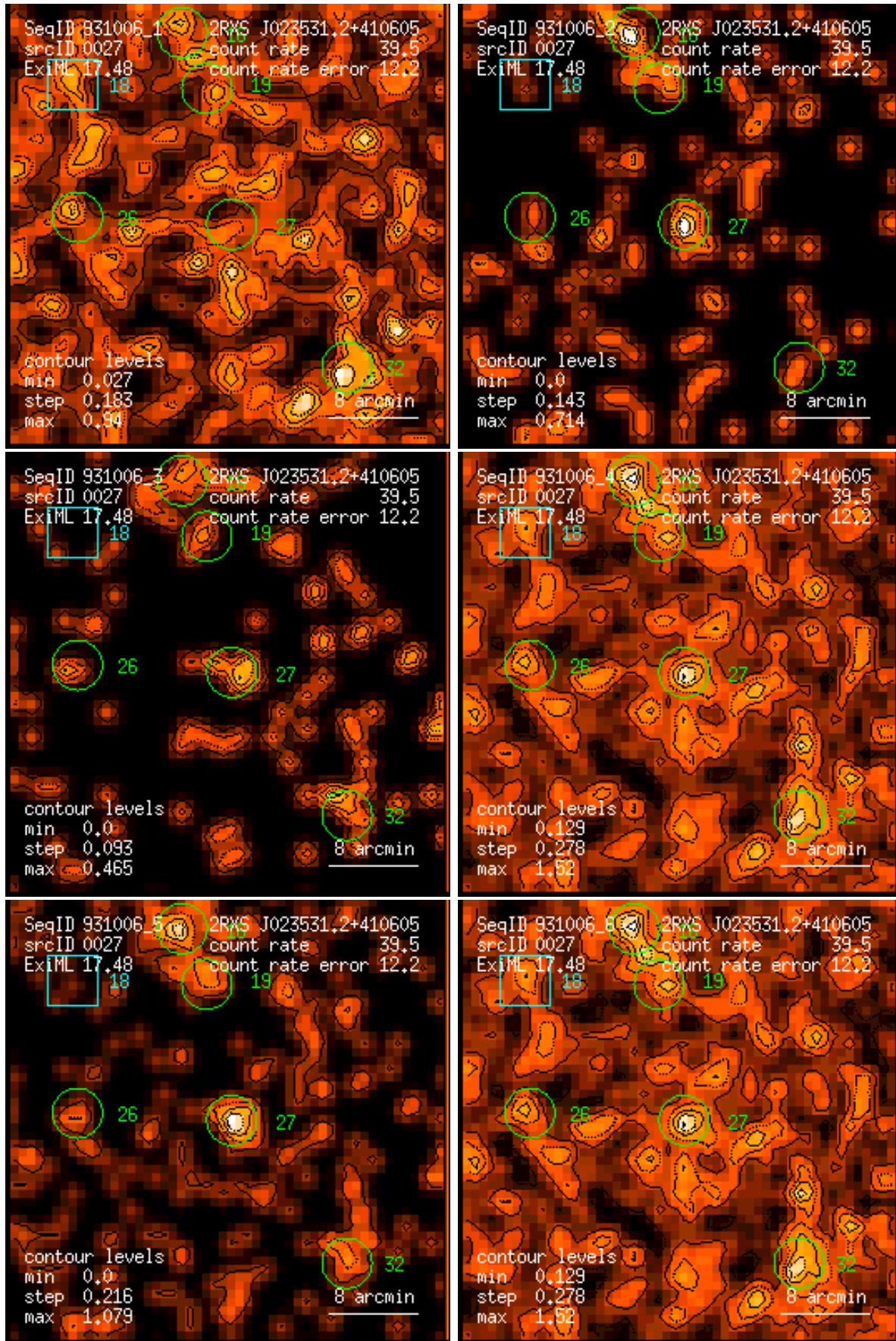
Figure 27: RASS 931006: detection 0027: band rate images, Gaussian filter: (1) PSPC channels 11 – 41, (2) 52 – 90, (3) 91 – 201, (4) 11 – 235, (5) 52 – 201, (6) 11 – 201. Broad band rates in counts/ks. Band rate contour levels in counts/ks/arcmin 2 .
