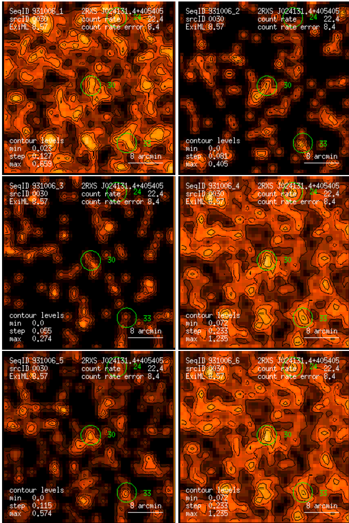
Figure 30: RASS 931006: detection 0030: band rate images, Gaussian filter: (1) PSPC channels 11 – 41, (2) 52 – 90, (3) 91 – 201, (4) 11 – 235, (5) 52 – 201, (6) 11 – 201. Broad band rates in counts/ks. Band rate contour levels in counts/ks/arcmin 2 .
