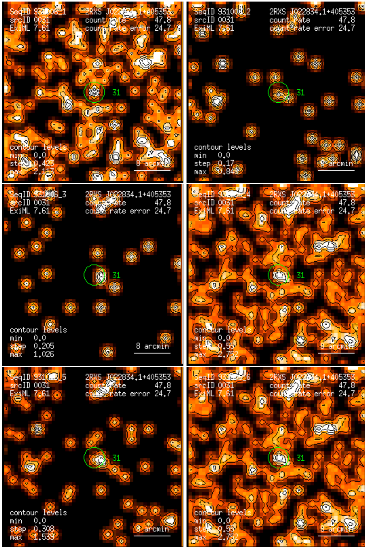
Figure 31: RASS 931006: detection 0031: band rate images, Gaussian filter: (1) PSPC channels 11 – 41, (2) 52 – 90, (3) 91 – 201, (4) 11 – 235, (5) 52 – 201, (6) 11 – 201. Broad band rates in counts/ks. Band rate contour levels in counts/ks/arcmin 2 .
