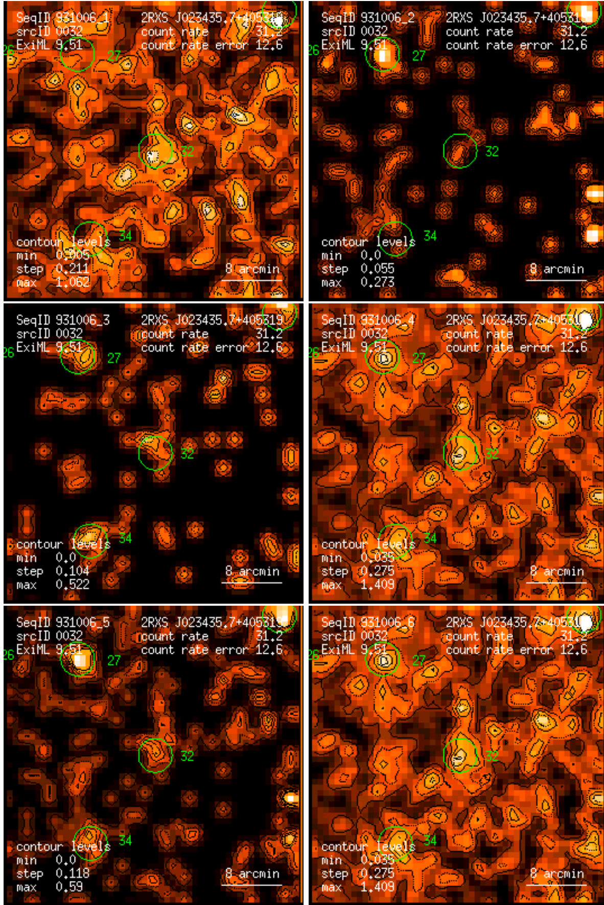
Figure 32: RASS 931006: detection 0032: band rate images, Gaussian filter: (1) PSPC channels 11 – 41, (2) 52 – 90, (3) 91 – 201, (4) 11 – 235, (5) 52 – 201, (6) 11 – 201. Broad band rates in counts/ks. Band rate contour levels in counts/ks/arcmin 2 .
