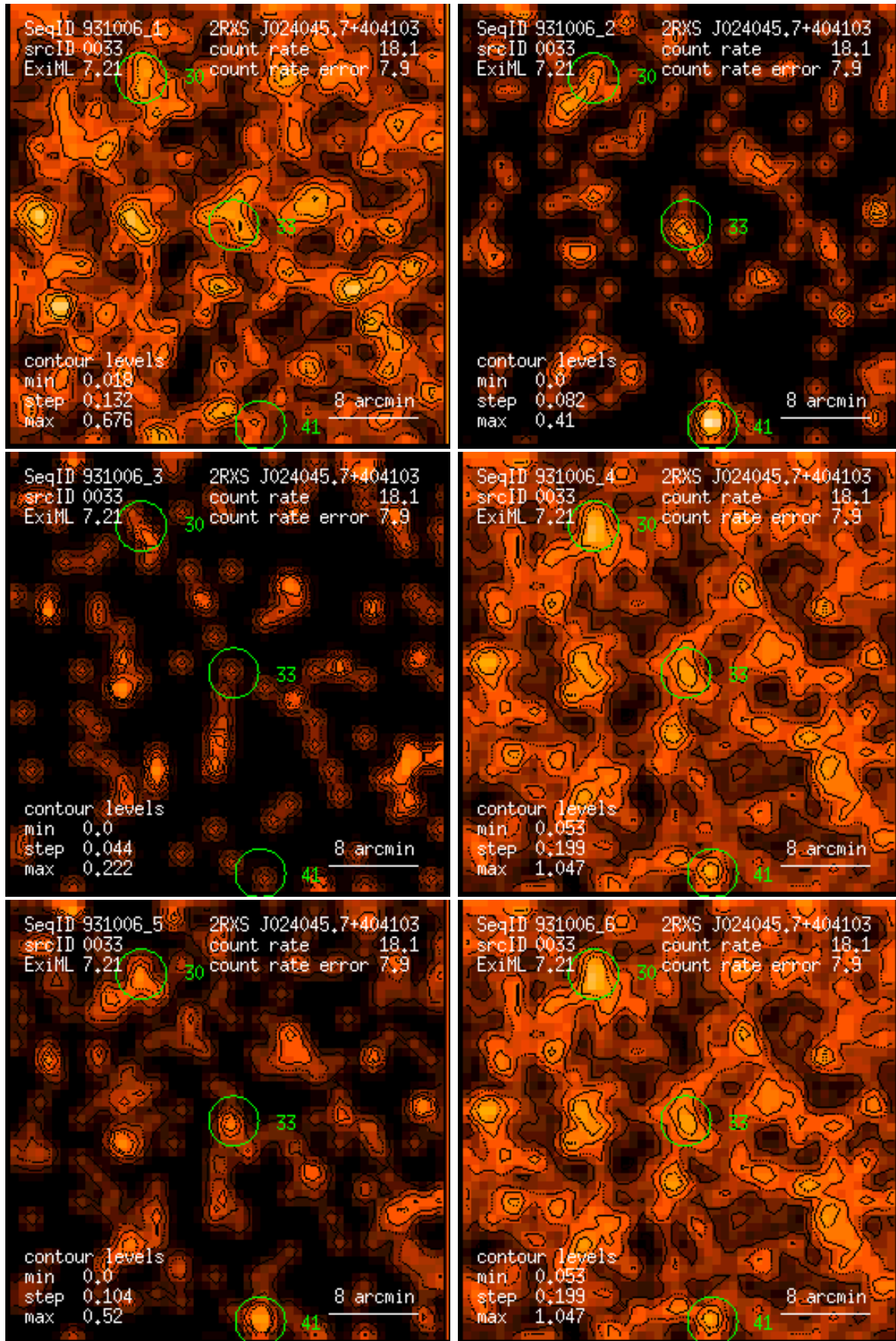
Figure 33: RASS 931006: detection 0033: band rate images, Gaussian filter: (1) PSPC channels 11 – 41, (2) 52 – 90, (3) 91 – 201, (4) 11 – 235, (5) 52 – 201, (6) 11 – 201. Broad band rates in counts/ks. Band rate contour levels in counts/ks/arcmin 2 .
