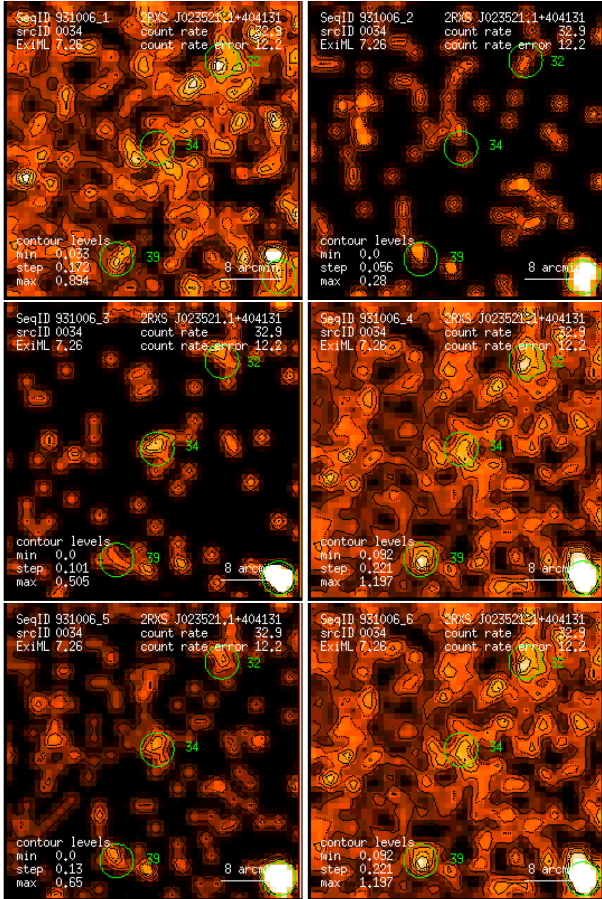
Figure 34: RASS 931006: detection 0034: band rate images, Gaussian filter: (1) PSPC channels 11 – 41, (2) 52 – 90, (3) 91 – 201, (4) 11 – 235, (5) 52 – 201, (6) 11 – 201. Broad band rates in counts/ks. Band rate contour levels in counts/ks/arcmin 2 .
