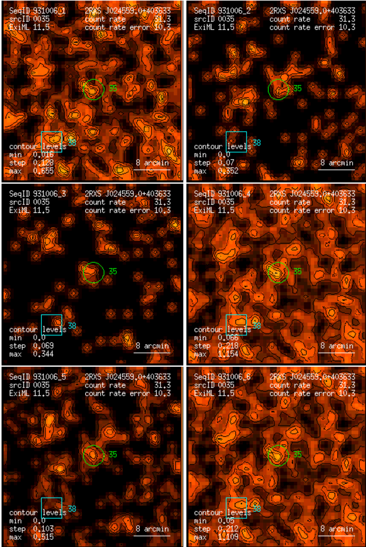
Figure 35: RASS 931006: detection 0035: band rate images, Gaussian filter: (1) PSPC channels 11 – 41, (2) 52 – 90, (3) 91 – 201, (4) 11 – 235, (5) 52 – 201, (6) 11 – 201. Broad band rates in counts/ks. Band rate contour levels in counts/ks/arcmin 2 .
