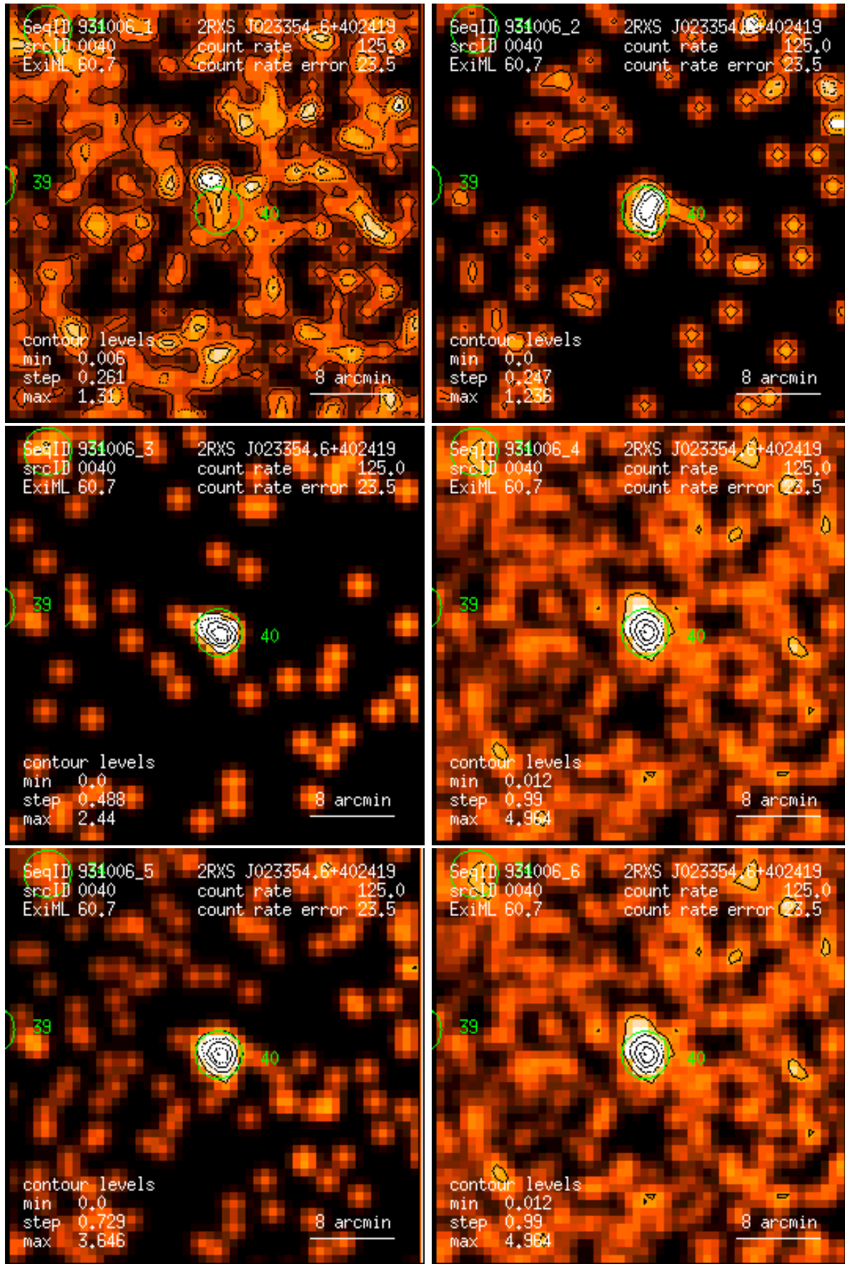
Figure 40: RASS 931006: detection 0040: band rate images, Gaussian filter: (1) PSPC channels 11 – 41, (2) 52 – 90, (3) 91 – 201, (4) 11 – 235, (5) 52 – 201, (6) 11 – 201. Broad band rates in counts/ks. Band rate contour levels in counts/ks/arcmin 2 .
