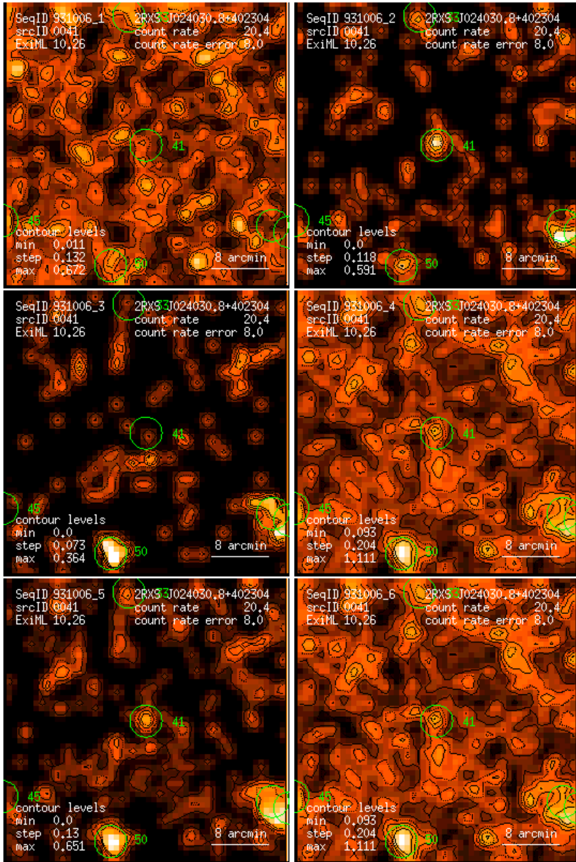
Figure 41: RASS 931006: detection 0041: band rate images, Gaussian filter: (1) PSPC channels 11 – 41, (2) 52 – 90, (3) 91 – 201, (4) 11 – 235, (5) 52 – 201, (6) 11 – 201. Broad band rates in counts/ks. Band rate contour levels in counts/ks/arcmin 2 .
