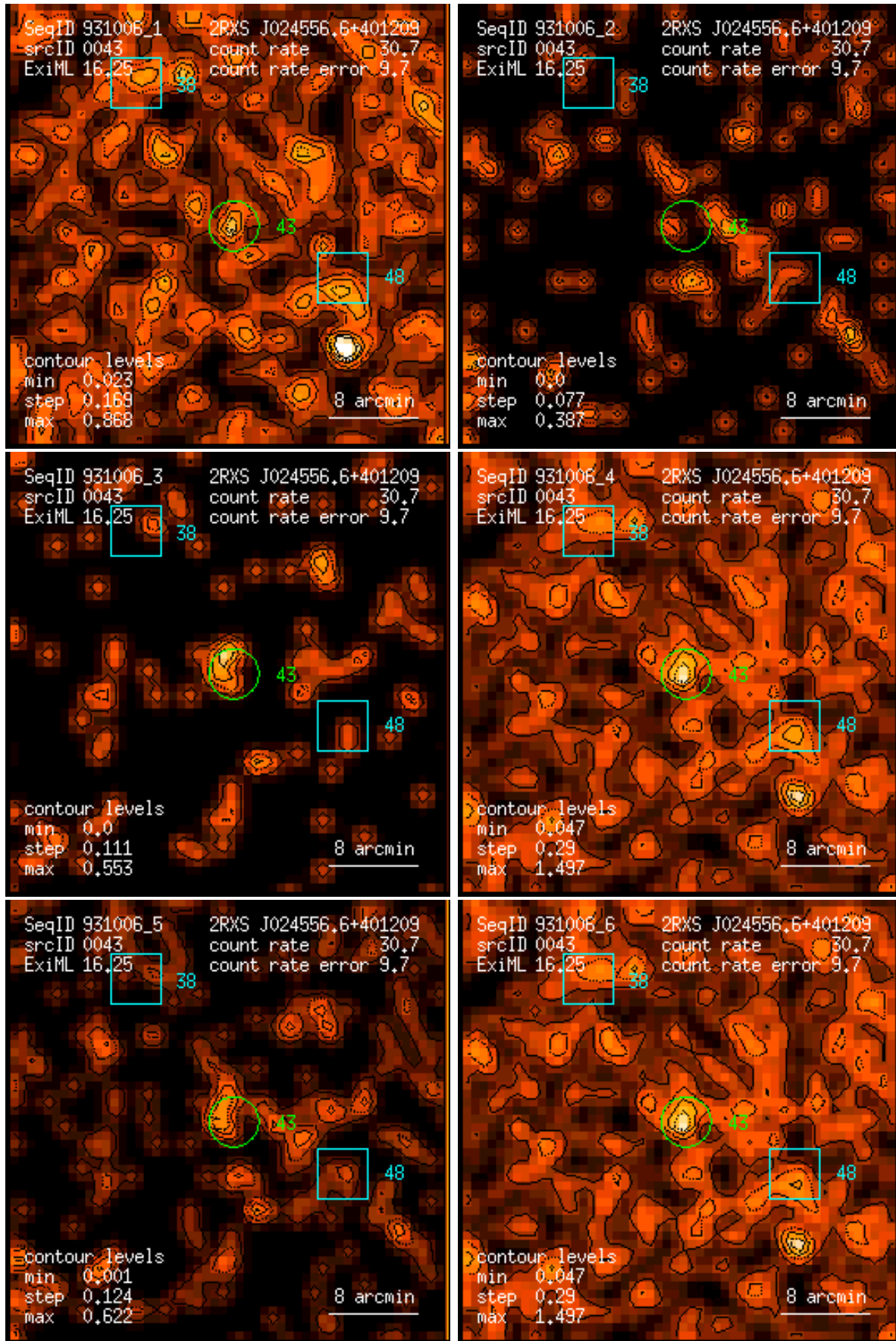
Figure 43: RASS 931006: detection 0043: band rate images, Gaussian filter: (1) PSPC channels 11 – 41, (2) 52 – 90, (3) 91 – 201, (4) 11 – 235, (5) 52 – 201, (6) 11 – 201. Broad band rates in counts/ks. Band rate contour levels in counts/ks/arcmin 2 .
