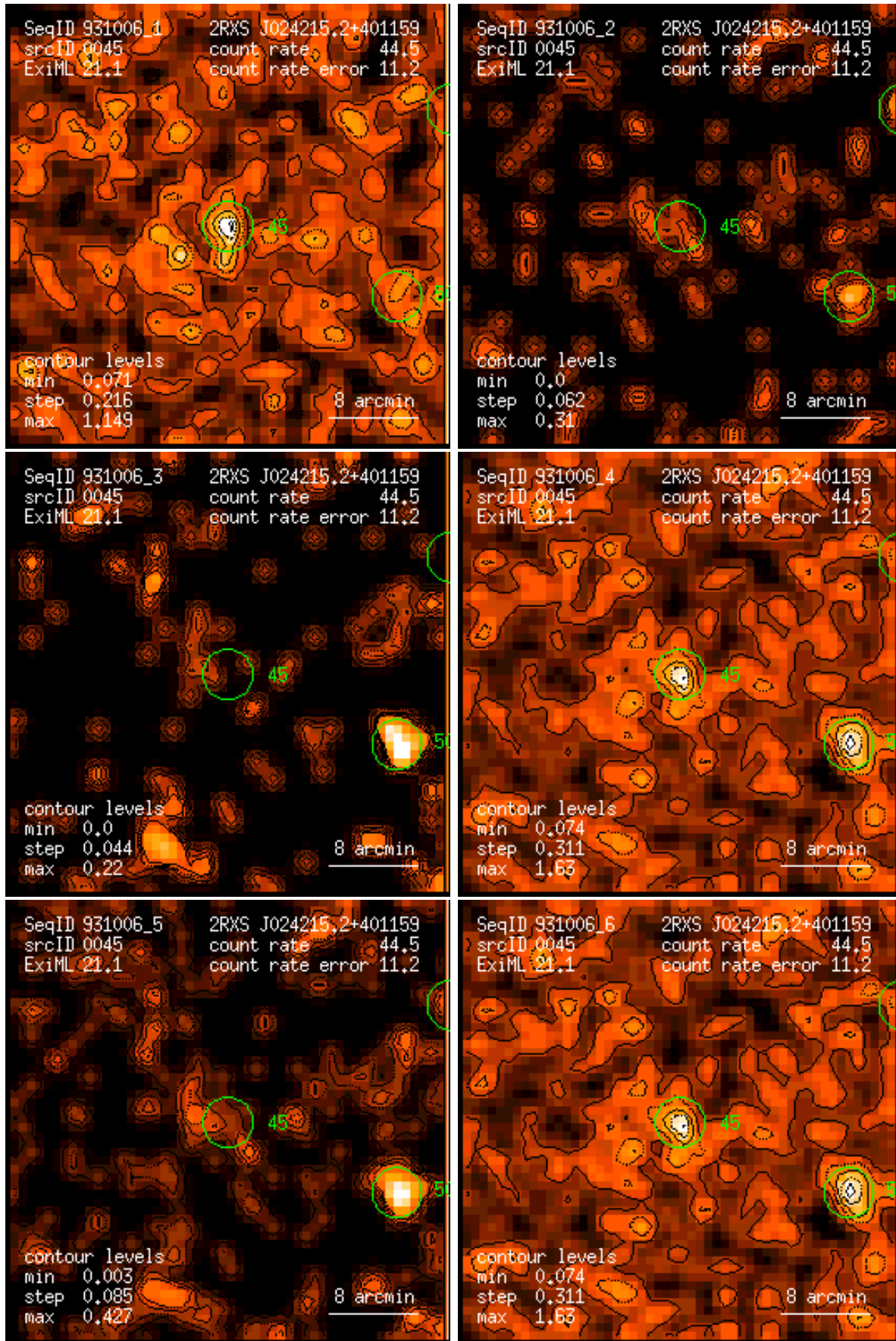
Figure 45: RASS 931006: detection 0045: band rate images, Gaussian filter: (1) PSPC channels 11 – 41, (2) 52 – 90, (3) 91 – 201, (4) 11 – 235, (5) 52 – 201, (6) 11 – 201. Broad band rates in counts/ks. Band rate contour levels in counts/ks/arcmin 2 .
