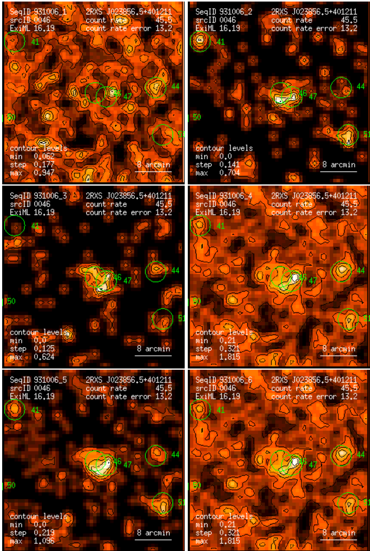
Figure 46: RASS 931006: detection 0046: band rate images, Gaussian filter: (1) PSPC channels 11 – 41, (2) 52 – 90, (3) 91 – 201, (4) 11 – 235, (5) 52 – 201, (6) 11 – 201. Broad band rates in counts/ks. Band rate contour levels in counts/ks/arcmin 2 .
