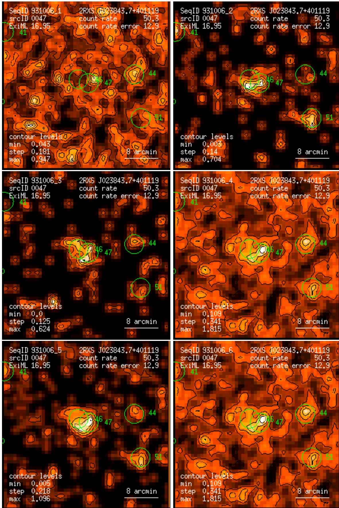
Figure 47: RASS 931006: detection 0047: band rate images, Gaussian filter: (1) PSPC channels 11 – 41, (2) 52 – 90, (3) 91 – 201, (4) 11 – 235, (5) 52 – 201, (6) 11 – 201. Broad band rates in counts/ks. Band rate contour levels in counts/ks/arcmin 2 .
