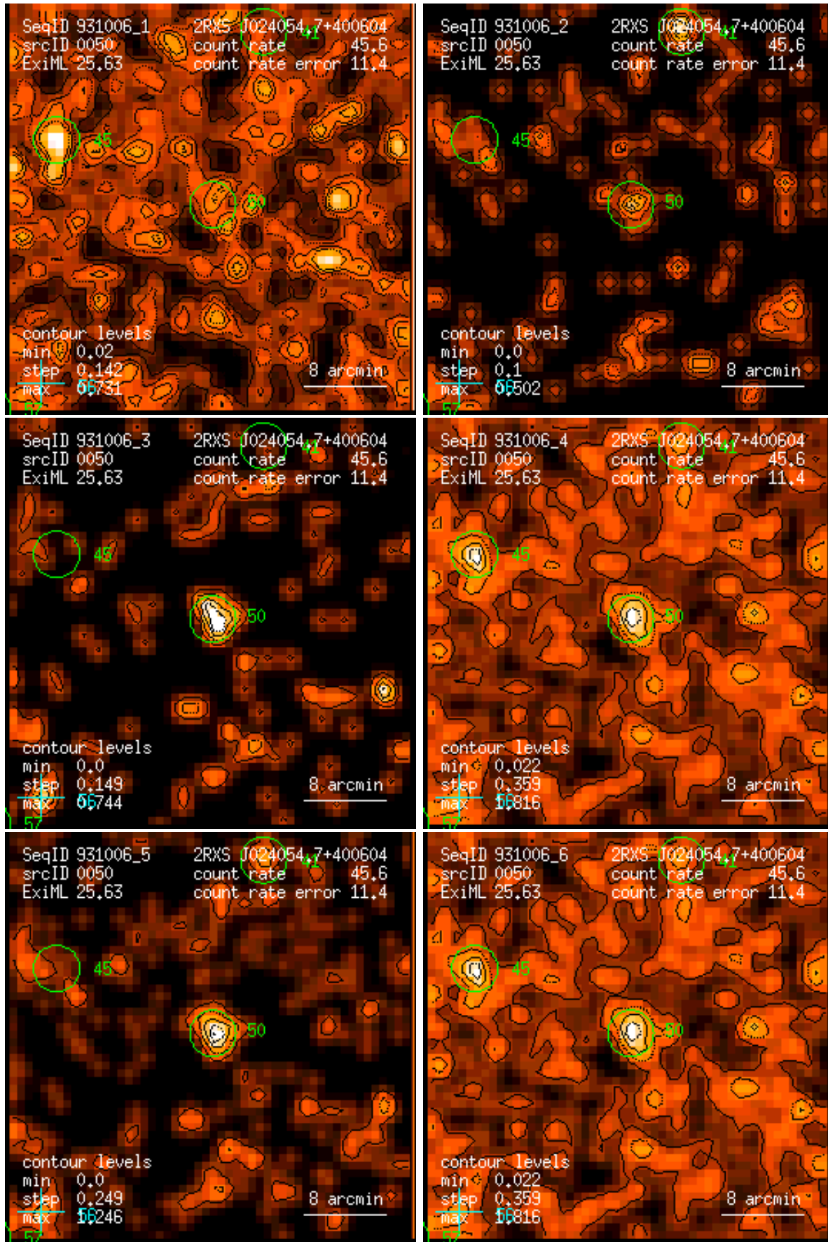
Figure 50: RASS 931006: detection 0050: band rate images, Gaussian filter: (1) PSPC channels 11 – 41, (2) 52 – 90, (3) 91 – 201, (4) 11 – 235, (5) 52 – 201, (6) 11 – 201. Broad band rates in counts/ks. Band rate contour levels in counts/ks/arcmin 2 .
