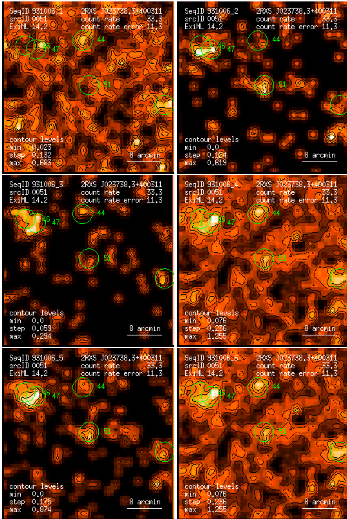
Figure 51: RASS 931006: detection 0051: band rate images, Gaussian filter: (1) PSPC channels 11 – 41, (2) 52 – 90, (3) 91 – 201, (4) 11 – 235, (5) 52 – 201, (6) 11 – 201. Broad band rates in counts/ks. Band rate contour levels in counts/ks/arcmin 2 .
